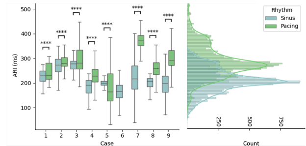
Figure 3. Distribution of rhythm-stratified ARI values per case (left) and the combined distribution (right). **** indicates p-value < 1e-4 . Boxplots show quartiles and median values.
