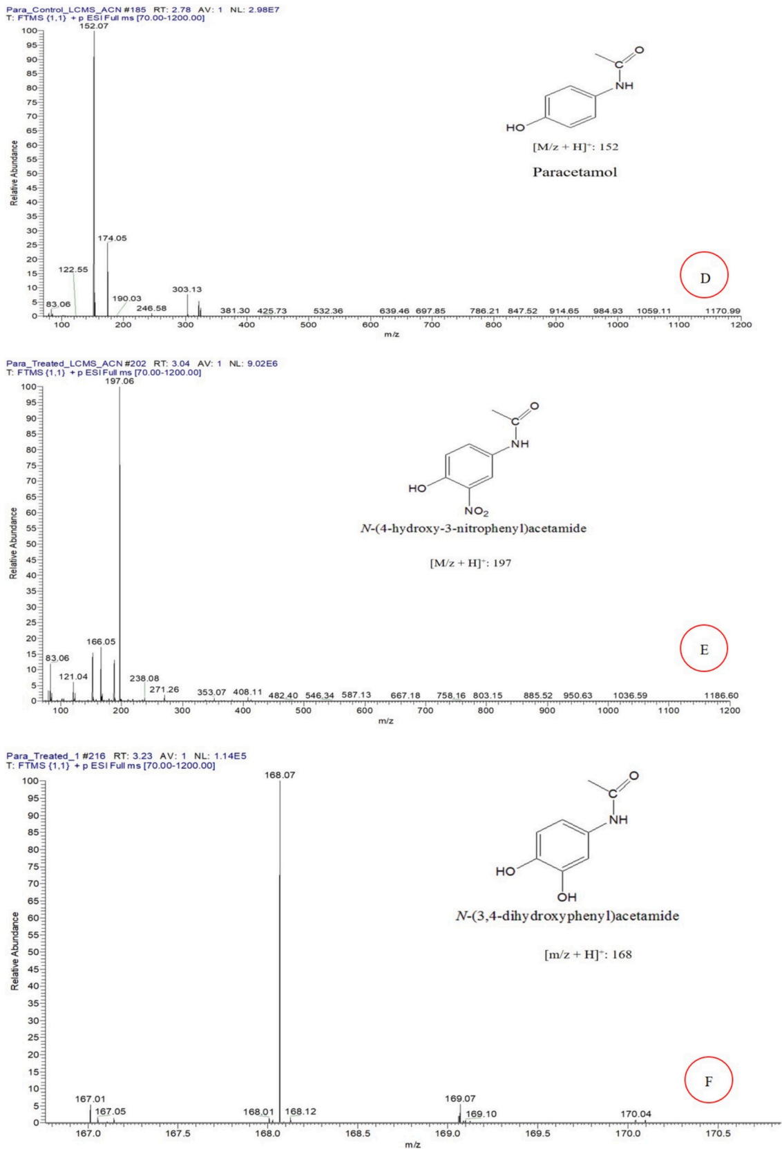
Fig. 8. Up (D): (Left) LC-MS fragments of paracetamol solubilized in acetonitrile (ACN) and Water. Middle (E): LC-MS fragment of the oxidation by-product 3 identified in the dry extract solubilized ACN. Bottom(F): LC-MS fragments of the oxidation by-product 4 identified in the water-solubilized dry extract.
