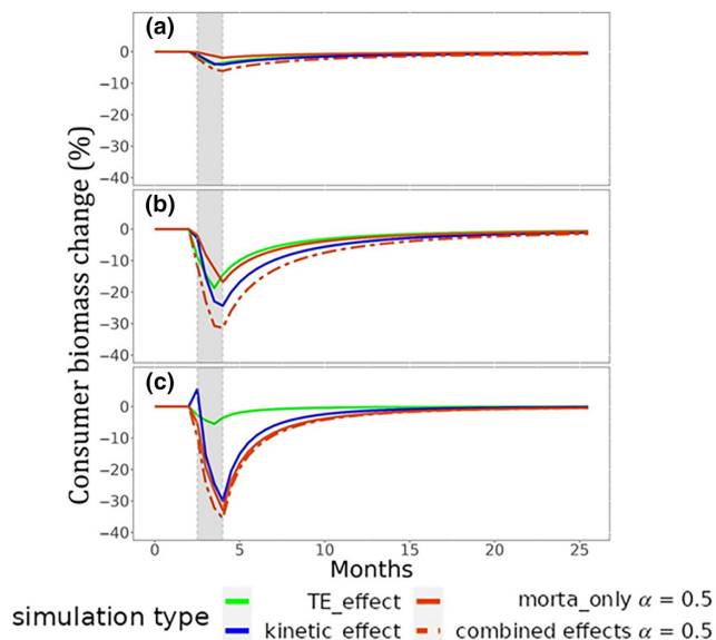
FIGURE 4 Instantaneous total consumer biomass response to an MHW occurrence: Simulation of a 1.5 month duration Category 3 MHW. The unique transfer efficiency effect, unique kinetic effect, \alpha=0.5 , and combined effects are green, blue, orange and dashed orange, respectively. Grey shade areas correspond to the MHW duration. With (a), (b) and (c) corresponding to polar, temperate and tropical biome simulation, respectively.
