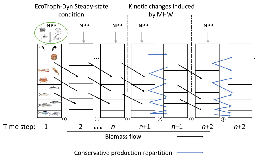
FIGURE 1 EcoTroph-Dyn scheme: The trophic functioning of marine food webs is represented by a biomass flow, with biomass entering the system at trophic level 1 due to net primary production (NPP). Biomass flow reaching each trophic level is then defined by the trophic transfer efficiency. The flow kinetic, temperature and MHW-dependant, is a key parameter to define boundaries of trophic classes and to derive the biomass at each trophic level and time step of the model from the biomass flow. Vertical dashed lines refer to an MHW occurrence, the black arrow represents biomass flow between trophic classes and time step, and the blue arrow represents production redistribution across trophic class boundaries due to an MHW. ① and ② refer to no MHW versus MHW effect, respectively (step 1 and step 2 in the paragraph above).
