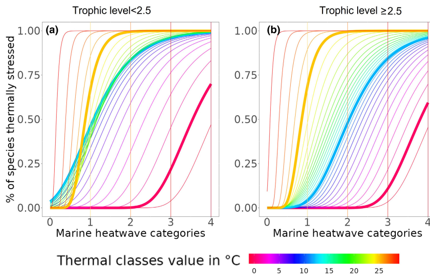
FIGURE 3 Proportion of species undergoing thermal stress: Thermal stress-based algorithm, with the reactions of trophic levels ( < and \geq ) 2.5 to a MHW event displayed on the (a) and (b) panels, respectively. Vertical lines from left to right correspond to MHW Category 1, Category 2, Category 3 and Category 4, respectively. Thicker lines correspond to the temperature used to simulate polar, temperate and tropical biomes in pink, blue and yellow, respectively.
