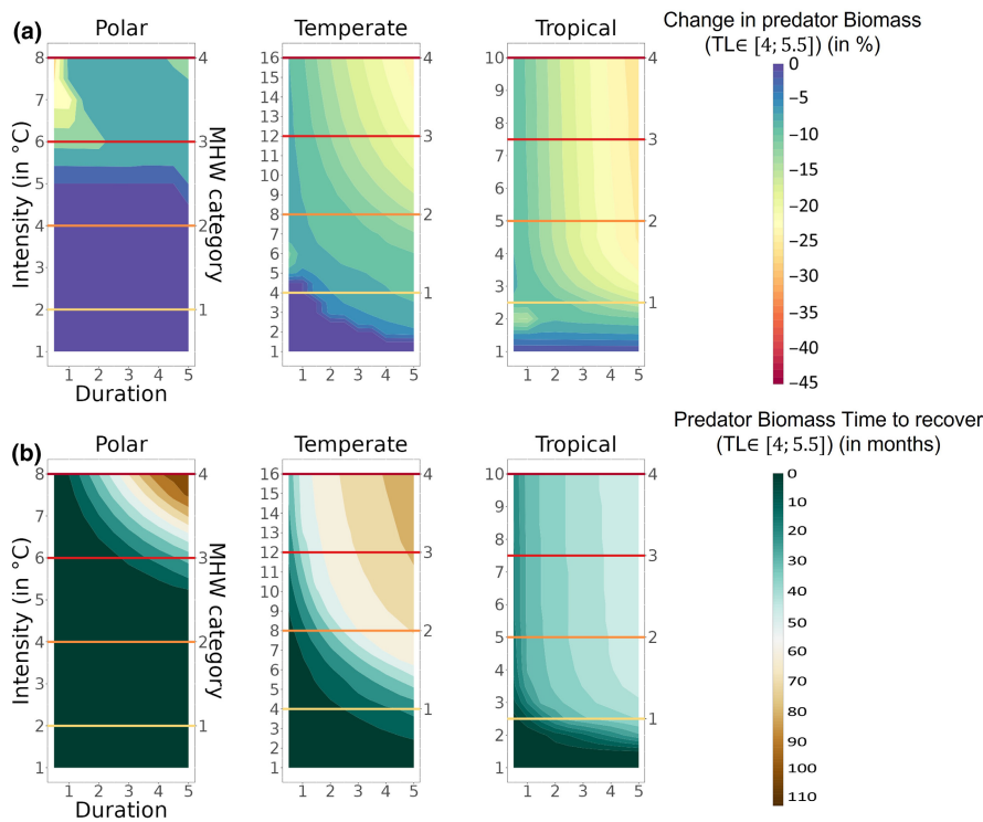
FIGURE 7 High TLs Average biomass loss and time to recover associated with MHWs characteristics with \alpha=0.5 : (a) corresponds to the average predator consumer biomass loss over the period of disturbance, and (b) is the necessary time for predator consumer biomass of each biome to recover 95% of pre-MHW-event biomass. Horizontal lines correspond to MHWs categories in each biome. The left-hand y-axis corresponds to the intensity of the MHWs in degrees Celsius, while the right-hand y-axis corresponds to the category of MHWs. The unit of MHWs duration on the x-axis is months.
