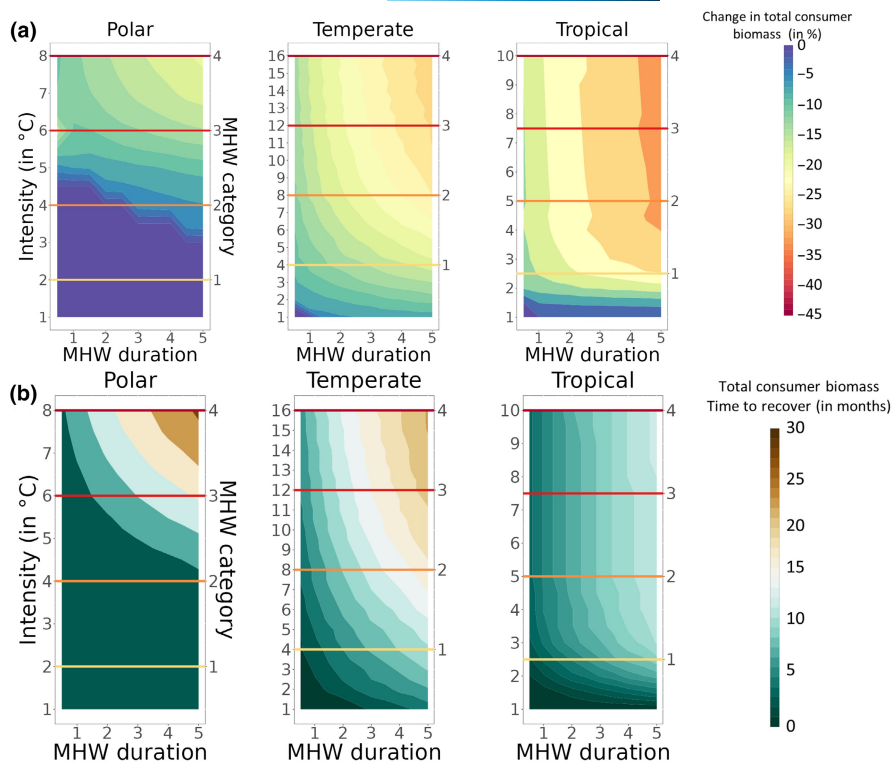
FIGURE 5 Average biomass loss and time to recover associated with MHWs characteristics with \alpha=0.5 : (a) corresponds to the average total consumer biomass loss over the period of disturbance, and (b) is the necessary time for the biome to recover 95% of pre-MHW-event biomass. Horizontal lines correspond to the simulated MHW's category in each biome. The left-hand y-axis corresponds to the intensity of the MHW in degrees Celsius, while the right-hand y-axis corresponds to the category of MHW. The unit of MHW duration on the x-axis is months.
