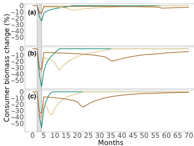
FIGURE 6 Instantaneous biomass changes per trophic group in response to a Category 3 and 1.5 month duration MHW in temperate biome with \alpha=0.5 : With low TLs biomass change, medium TL biomass change and high TL biomass change, represented in green, light brown and dark brown respectively. Polar, temperate and tropical biomes correspond to the (a), (b) and (c) panels, respectively.
