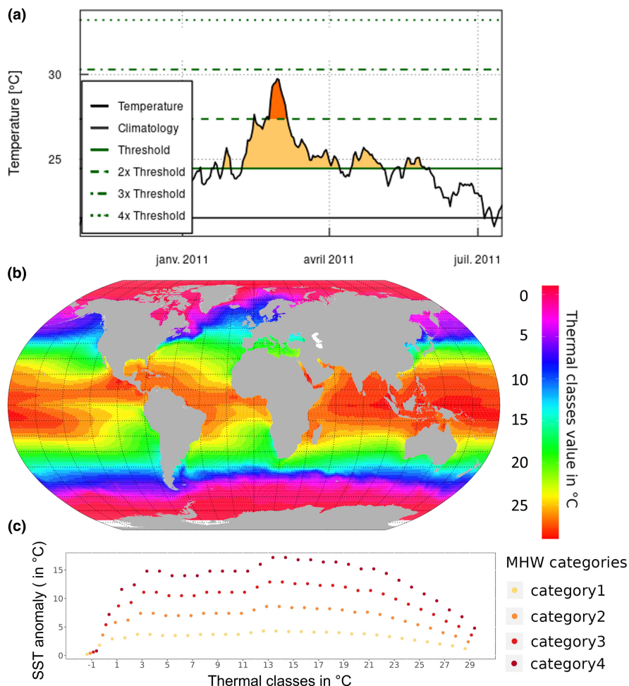
FIGURE 2 MHWs detection and category threshold characteristics across the world ocean and map of ocean averaged temperature by thermal classes: (a) Schematic explanation of MHWs detection for a spatial cell. The solid horizontal green and black lines represent the extreme threshold value and the reference temperature, respectively. (b) A map of thermal classes of 1^\circ\text{C} intervals from -1 to 29^\circ\text{C} categorised based on the reference temperature at each spatial cell. (c) Average MHW's category threshold per thermal class.
