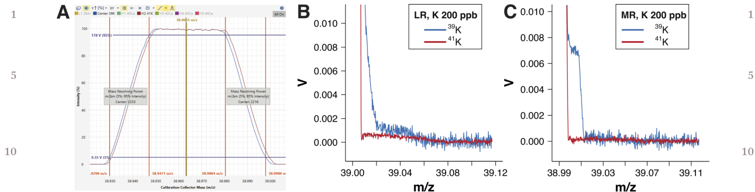
Fig. 2 (A) Peak scan in the low-resolution mode of the SRM-3141a solution at 200 \text{ ng mL}^{-1} (K 200 ppb) using the set of parameters given in Table 1 showing the peak shape of the m/z -values 39 and 41 (blue and red, respectively) with the automated calculation of the resolution (5 95% of m/z -value 39) on the ascending edge of the peak. (B) Details of the interferences in the low-resolution mode on the high mass shoulder of the m/z -values 39 and 41. (C) Details of the interferences in the medium-resolution mode on the high mass shoulder of the m/z -values 39 and 41.
