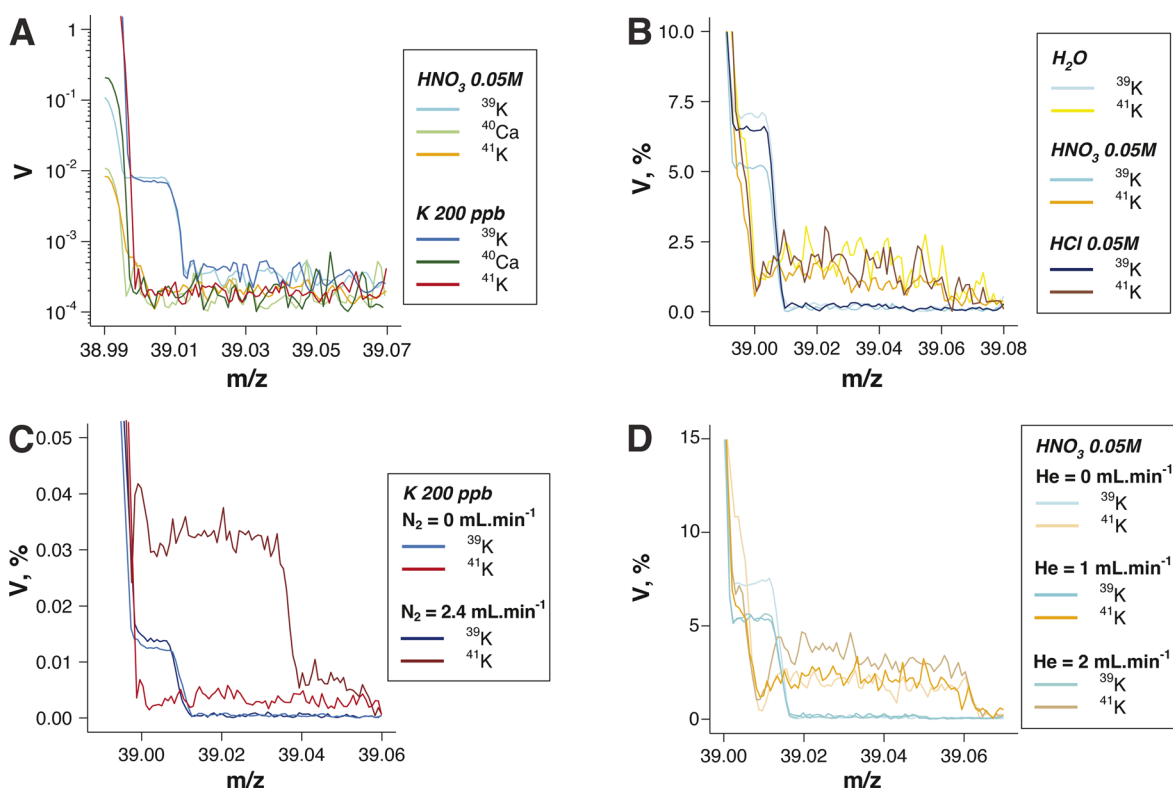
Fig. 3 (A) Details of the interferences in the medium-resolution mode on the high mass shoulder of the m/z -values 39, 40 and 41 as a function of K concentration. Details of interferences relative intensities in the medium-resolution mode on the high mass shoulder of the m/z -values 39 and 41: (B) as a function of the nature of the solution; (C) as a function of the presence of \text{N}_2 in the Apex Omega desolvator; (D) as a function of the presence of He in the CRC.
