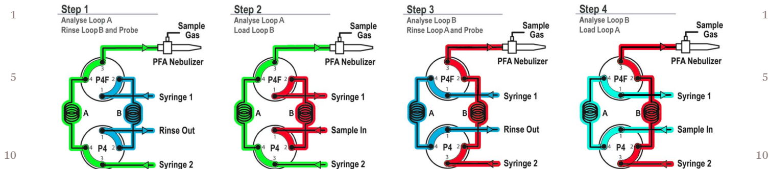
Fig. 1 Flow paths of the microFAST Isotope autosampler dual loop injection, composed of two loops (A and B), two syringes (1 and 2) and two 4-way valves (P4F and P4). The syringe 1 loads solutions while syringe 2 injects solutions at desired flow rate. During step 1, the sample solution (green) loaded in loop A is injected in the nebulizer, while the loop B is rinsed with the working solution (blue). During step 2, the sample solution (green) loaded in loop A is still injected in the nebulizer, but the loop B is now loading the new sample solution (red). During step 3, the two 4-way valves switch, such that the new sample (red) loaded in loop B is now injected, while the loop A is rinsed with the working solution (blue). During step 4, the sample solution (red) loaded in loop A is still injected in the nebulizer, but the loop B is now loading the new sample solution (cyan). Adapted from ESI©.
