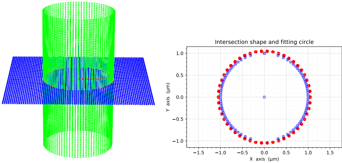
Fig. 3: Intersection between a plane (without inclination) and a cylinder: intersection shape (in blue) and fitted circle (in red, radius: 1.04 \mu\text{m} ).
