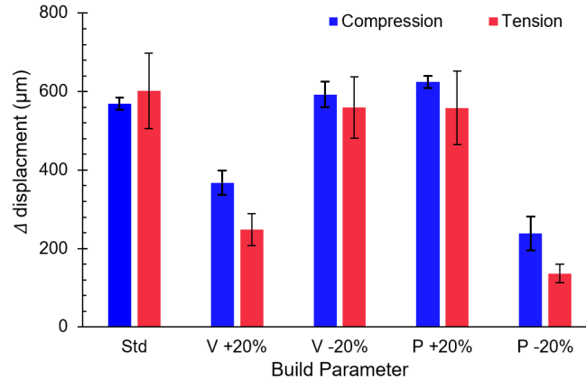
Figure 9 – Comparison between the compressive and tensile displacements for the build configurations. The load wedge location is related to the compressive displacement and the crack tip is associated with the tensile displacement (the error bars are computed from the data dispersion shown in Figure 8)
