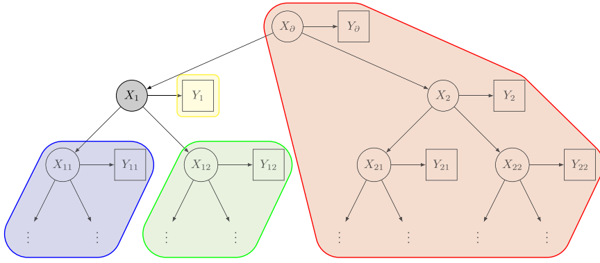
Fig 2. Illustration of the Markov property for the HMT. Conditioning on X_1 (in grey) implies that the HMT process (X, Y) becomes independent between the four connected components of variable-dependence tree from Figure 1 where the vertex X_1 is removed, that is, Y_1 , (X_{T(11)}, Y_{T(11)}) , (X_{T(12)}, Y_{T(12)}) and (X_{T \setminus T(1)}, Y_{T \setminus T(1)}) (respectively in yellow, blue, green and red) are independent conditionally on X_1 .
