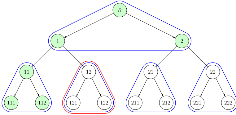
Fig 5. Illustration of the “past” subtree \Delta^*(T(u, m), k) of the block subtree T(u, m) for m = 1 , u = 12 and k = 1 . The block subtrees are circled with blue lines, and the block subtree T(12, 1) is circled a second time with a red line. The vertices in green are those in \Delta^*(T(12, 1), 1) . Note the difference with \Delta(u', k') , e.g. vertex 111 is in \Delta^*(T(12, 1), 1) but not in \Delta^*(12, 2) , and vertex 21 is in \Delta^*(121, 3) but not in \Delta^*(T(12, 1), 1) .
