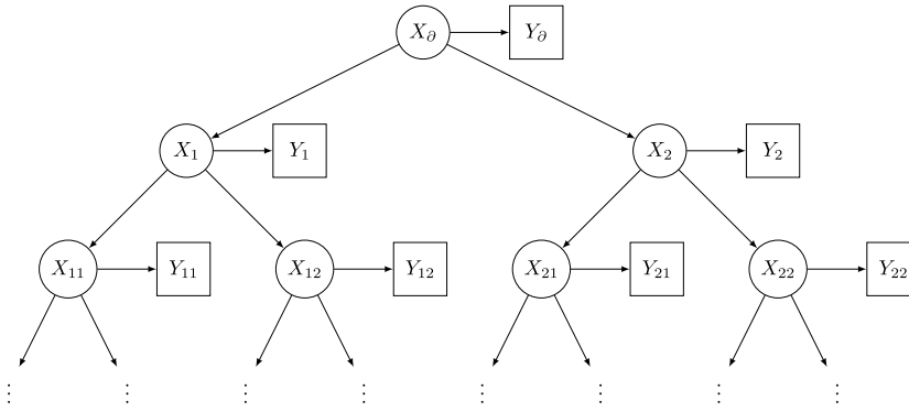
Fig 1. Graph of dependence for variables of a HMT process indexed by the complete infinite rooted binary tree T . The observed variables are represented inside square, while the hidden variables are represented inside circles.
