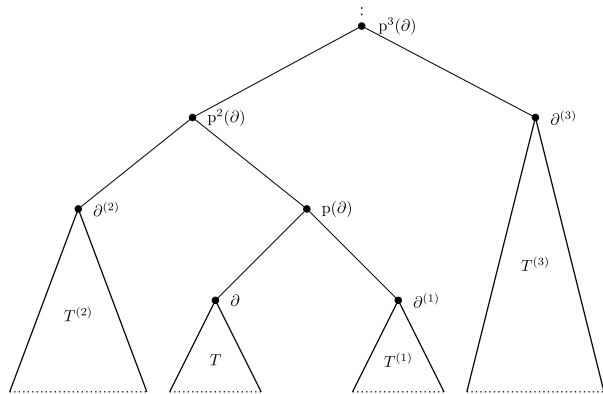
Fig 4. Illustration of the construction of the extended random plane rooted tree T^\infty (which is rooted at \partial ) for \mathcal{U}_{(-1)} = 0 and \mathcal{U}_{(-2)} = 1 .
