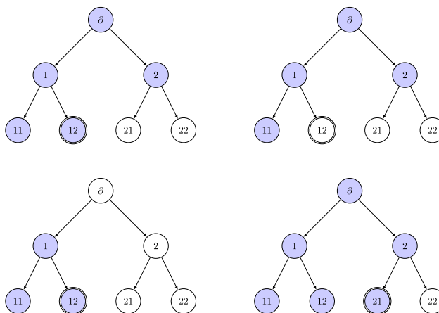
Fig 3. Illustration of the subtrees \Delta(u, k) and \Delta^*(u, k) where vertices in \Delta(u, k) and \Delta^*(u, k) are in blue and the vertex u is inside a double circle. From left to right and top to bottom, using Neveu's notation, we have \Delta(12) = \Delta(12, 2) , \Delta^*(12) = \Delta^*(12, 2) , \Delta(12, 1) and \Delta(21) = \Delta(21, 2) . Note that \Delta(12) and \Delta(21) have a different number of vertices, while vertices 12 and 21 are in the same generation.
