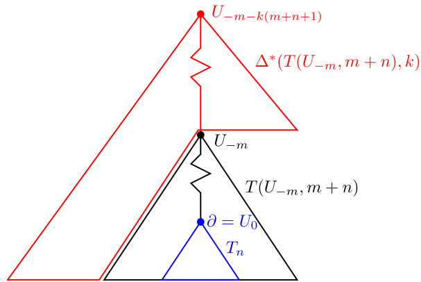
Fig 6. Illustration of the gap in (38) between the variables (Y_v, v \in T_n) (bottom triangle in blue) and the variables (Y_v, v \in \Delta^*(T(U_{-m}, m+n), k)) and X_{p^{k(m+n+1)}(U_{-m})} that appear in the conditioning (top partial triangle in red). Note that the two groups of variables are separated by the path from U_{-m-1} = p(U_{-m}) to \partial = U_0 , which is of length m+1 .
