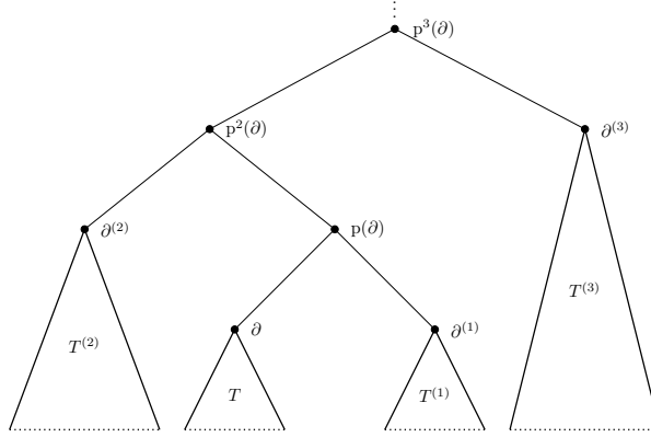
Figure 4: Illustration of the construction of the extended random plane rooted tree T^\infty (which is rooted at \partial ) for \mathcal{U}_{(-1)} = 0 and \mathcal{U}_{(-2)} = 1 .
