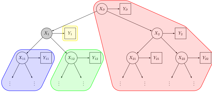
Figure 2: Illustration of the Markov property for the HMT. Conditioning on X_1 (in grey) implies that the HMT process (X, Y) becomes independent between the four connected components of variable-dependence tree from Figure 1 where the vertex X_1 is removed, that is, Y_1 , (X_{T(11)}, Y_{T(11)}) , (X_{T(12)}, Y_{T(12)}) and (X_{T \setminus T(1)}, Y_{T \setminus T(1)}) (respectively in yellow, blue, green and red) are independent conditionally on X_1 .
