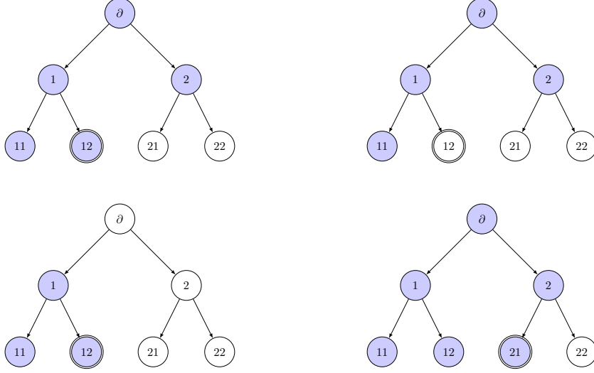
Figure 3: Illustration of the subtrees \Delta(u, k) and \Delta^*(u, k) where vertices in \Delta(u, k) and \Delta^*(u, k) are in blue and the vertex u is inside a double circle. From left to right and top to bottom, using Neveu's notation, we have \Delta(12) = \Delta(12, 2) , \Delta^*(12) = \Delta^*(12, 2) , \Delta(12, 1) and \Delta(21) = \Delta(21, 2) . Note that \Delta(12) and \Delta(21) have a different number of vertices, while vertices 12 and 21 are in the same generation.
