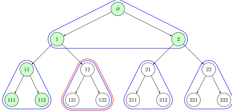
Figure 5: Illustration of the “past” subtree \Delta^*(T(u, m), k) of the block subtree T(u, m) for m = 1 , u = 12 and k = 1 . The block subtrees are circled with blue lines, and the block subtree T(12, 1) is circled a second time with a red line. The vertices in green are those in \Delta^*(T(12, 1), 1) . Note the difference with \Delta(u', k') , e.g. vertex 111 is in \Delta^*(T(12, 1), 1) but not in \Delta^*(12, 2) , and vertex 21 is in \Delta^*(121, 3) but not in \Delta^*(T(12, 1), 1) .
