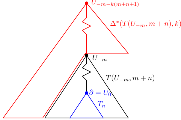
Figure 6: Illustration of the gap in (38) between the variables (Y_v, v \in T_n) (bottom triangle in blue) and the variables (Y_v, v \in \Delta^*(T(U_{-m}, m+n), k)) and X_{\mathbf{p}^{k(m+n+1)}(U_{-m})} that appear in the conditioning (top partial triangle in red). Note that the two groups of variables are separated by the path from U_{-m-1} = \mathbf{p}(U_{-m}) to \partial = U_0 , which is of length m+1 .
