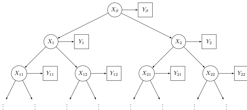
Figure 1: Graph of dependance for variables of a HMT process indexed by the complete infinite rooted binary tree T . The observed variables are represented inside square, while the hidden variables are represented inside circles.
