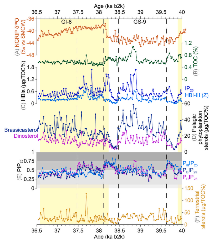
Fig. 3. Biomarker results from MD99-2304 with NGRIP oxygen isotopes as a reference. (A) NGRIP \delta^{18}\text{O} (‰ vs SMOW) (20 years mean, GIC05 age model) (North Greenland Ice Core Project members, 2004; Andersen et al., 2006), (B) TOC, (C) HBIs (IP 25 and HBI-III (Z)), (D) pelagic phytoplankton sterols (brassicasterol and dinosterol), (E) PIP 25 (P III IP 25 , P B IP 25 , and P D IP 25 ), and (f) terrestrial sterols (campesterol+ \beta -sitosterol). All records are plotted as ka b2k. Yellow bars indicate the GIs (i.e., GI-9 and GI-8) as defined in the NGRIP ice core (Rasmussen et al., 2014). Grey boxes stand for the classification of PIP 25 values (from darkest to lightest: 0.75–1 extensive sea ice, 0.5–0.75 seasonal ice/stable ice edge, and 0–0.5 reduced ice) (Müller et al., 2011; Xiao et al., 2015; Stein et al., 2017). The black dashed lines represent the divisions between different time periods based on the identified changes in concentrations of all biomarkers and PIP 25 values (the distribution of IP 25 and phytoplankton biomarker concentrations refers to Fig. 4).
