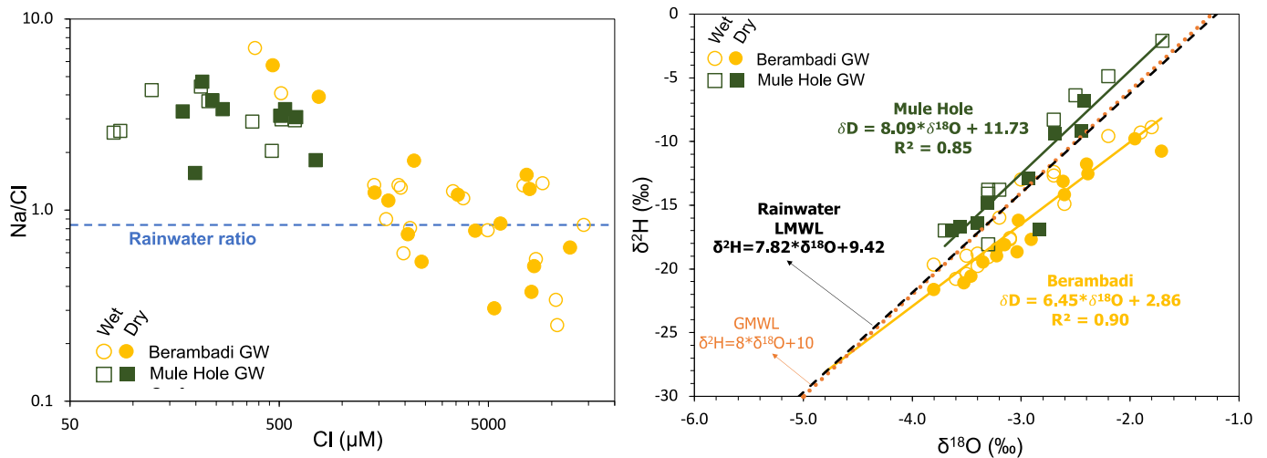
Fig. 2. The plot depicting, a) Na/Cl and Cl of groundwater, showing increasing Cl concentration and a concurrent reduction in Na/Cl ratio below the rainwater ratio of 0.81 (dashed line, Riote et al., 2014a), b) \delta^{18}\text{O} and \delta^2\text{H} bivariate plots for groundwater from Mule Hole and Berambadi along with the local meteoric water line (LMWL, black dashed line, Table S2) from local precipitation and global meteoric water line (GMWL, orange dashed line, Craig (1961)). Equations for the linear relationship between \delta^{18}\text{O} and \delta^2\text{H} for all groundwater from watershed across both season is shown.
