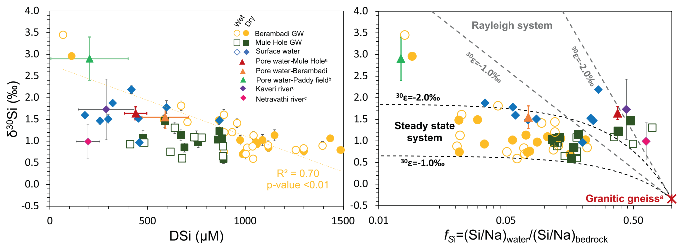
Fig. 4. The plot between \delta^{30}\text{Si} and a) dissolved silicon in groundwater and surface water from Mule Hole and Berambadi, (the error bar indicates 1SD), the regression line has been shown for Berambadi groundwater, b) Evolution of \delta^{30}\text{Si} with fraction of Si mobilized into dissolved phase ( f_{\text{Si}} ) during weathering (see section 2.5.2 for more details). Dashed and dotted lines represent the evolution of \delta^{30}\text{Si} expected from Si removal under two model scenarios: i) Rayleigh distillation from a finite Si pool, ii) steady-state open flow through model (Bouchez et al., 2013) (a: Riotte et al. (2018a), b: Riotte et al. (2018b), c: Sarath et al. (2022)).
