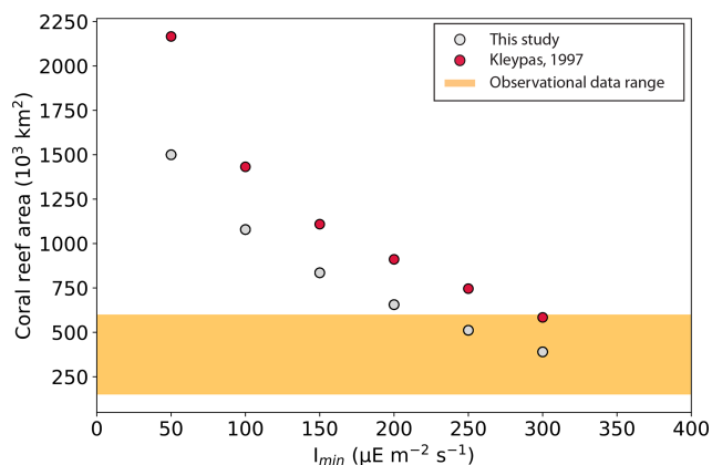
Figure 5. Global coral reef area ( 10^3 \text{ km}^2 ) simulated in this study and in Kleypas (1997) as a function of I_{\min} (the minimum light intensity necessary for reef growth, \mu\text{E m}^{-2} \text{s}^{-1} ). The range of observational data for the global coral reef area (Sect. 2.4) is shown with the yellow bar.
