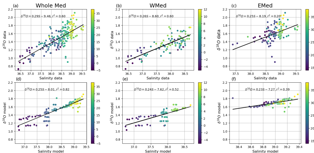
Figure 4. \delta^{18}\text{O}_w –salinity relationship in the surface water (average 0–200 m depth of the whole basin – a, d ; western basin – b, e ; and eastern basin – c, f ) calculated from available in situ data (Epstein and Mayeda, 1953; Stahl and Rinow, 1973; Pierre et al., 1986; Gat et al., 1996; Pierre, 1999) in the upper panel (in a–c ) and from model outputs extracted in the same positions of in situ data (in d–f ). The colour code indicates the longitude of the data in degrees east ( ^{\circ}\text{E} ).
