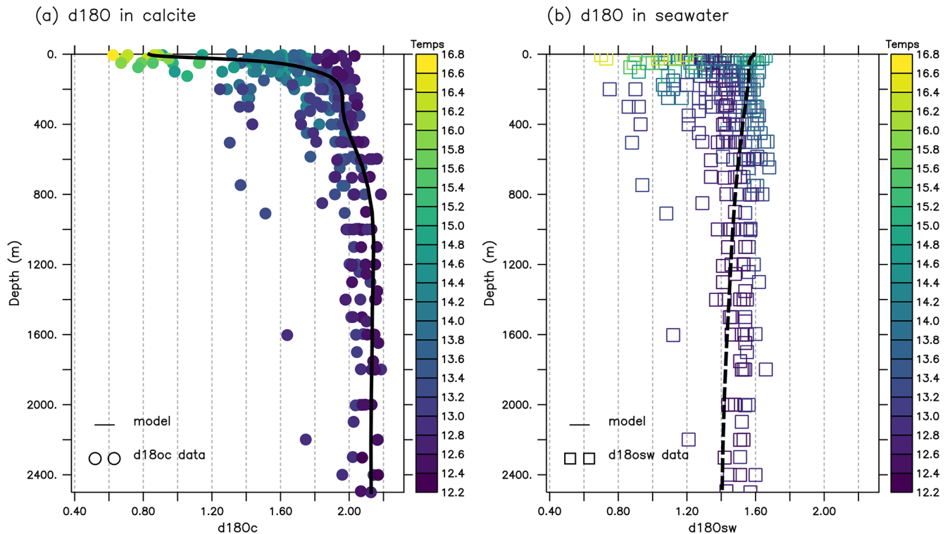
Figure A2. (a) Comparison of the simulated average vertical profiles of \delta^{18}\text{O}_c (in ‰) (circles represent data, and the line is from model outputs). (b) The same as (a) but for \delta^{18}\text{O}_w .
