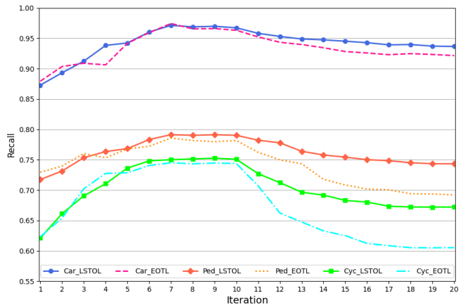
Fig. 5. Recall curves for cars, pedestrians, and cyclists during the system transfer from KITTI to Waymo.
