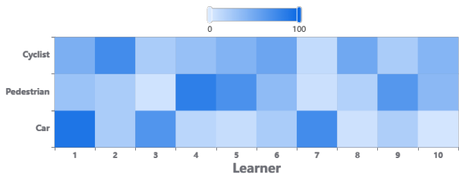
Fig. 6. Heatmap of “expert” opinions of each learner. Each column represents the distribution of high-confidence predictions for one learner across the test samples, while each row represents high-confidence results produced by different learners for the same class.
