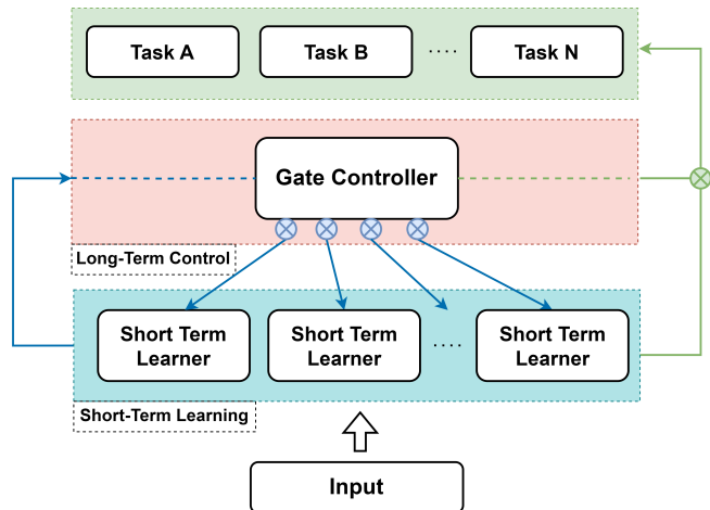
Fig. 1. Illustration of the Long-Short-Term Online Learning (LSTOL) framework which consists of two modules: short-term learning and long-term control. Input samples are first processed by a set of short-term learners for pre-prediction. The long-term control module collects these pre-prediction to calculate indicators for online prediction, then passes them to the Gate Controller to determine actions for each learner. During the learning phase (blue line), the module calculates the online loss to update the learner weights, which are used in the prediction phase (green line) to determine the object category.
