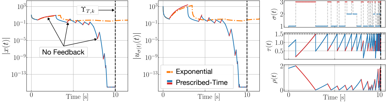
Figure 4: Comparison between controller with Exponential convergences and PT-Regulation with intermittent feedback. Left: Trajectory of system's state norm plotted in logarithmic scale. Center: Trajectories of the switching feedback law u_q . Right: Trajectories of the switching signal \sigma (top), the dwell-time state \tau (middle), and the monitor state \rho (bottom) for the PT-Regulation mechanism with intermittent feedback.
