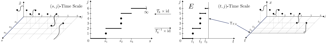
Figure 1: Dilation and contraction of hybrid time domains and hybrid arcs. The structure of the hybrid time domain E in the (t, j) -time scale is preserved under the diffeomorphism \mathcal{T}_k \times \text{id} in the (s, j) -time scale.
