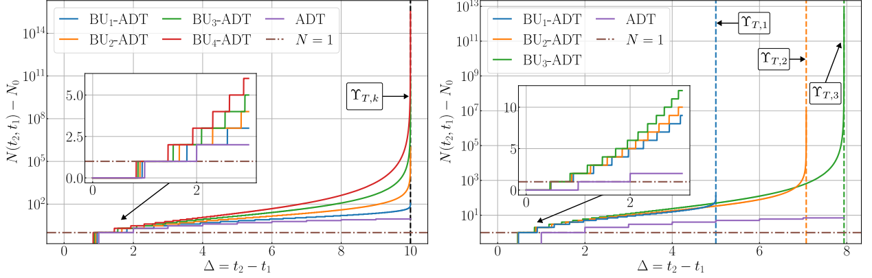
Figure 2: \text{BU}_k\text{-ADT} condition (22) for k \in \{1, 2, 3, 4\} . Left: When \mu_0 = 1 , T = 10 , and t_1 = 0 , there exists a single common terminal time T = \Upsilon_{T,k} for all k . Right: When \mu_0 = 2 , T = 10 , and t_1 = 0 , the dependence of \Upsilon_{T,k} on \mu_0 (see Proposition 1) leads to the emergence of three distinct terminal times.
