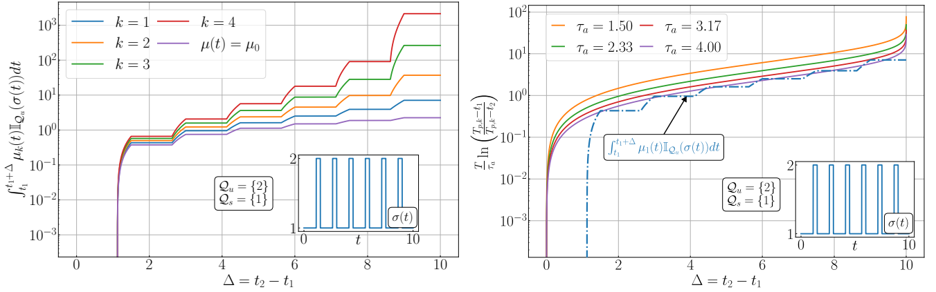
Figure 3: Functions appearing in the BU_k -AAT condition (36) using the switching signal \sigma(\cdot) (see inset), T = 10 , and \mu_0 = 1 .
