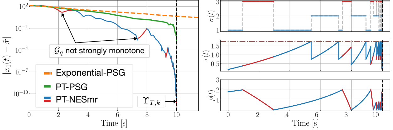
Figure 5: Comparison between Pseudo-Gradient Flow (PSG) with exponential convergence and PT Nash-Equilibrium Seeking in a Switching Game. Left: Trajectory of the errors to the NE generated by the PT-NESmr, the PT-PSG, and the Exponential PSG dynamics. Right: Trajectories of the switching signal \sigma(t) (top), the dwell-time state \tau (middle), and the monitor state \rho(t) (bottom) for the PT-NESmr dynamics.
