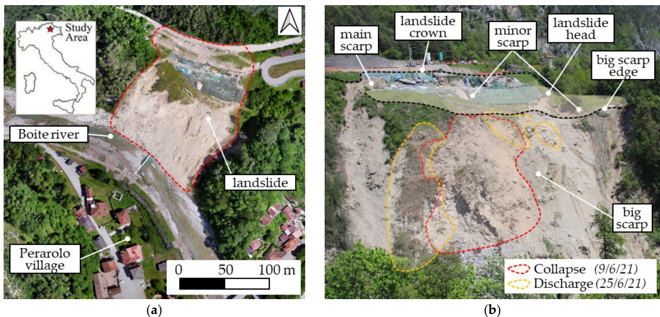
Figure 7. (a) Areal view of the Sant'Andrea landslide site and Perarolo di Cadore village (NE Italy) taken from UAV survey in March 2022; (b) front view of the slope on 8 June 2021 just before the collapse induced with explosives.
