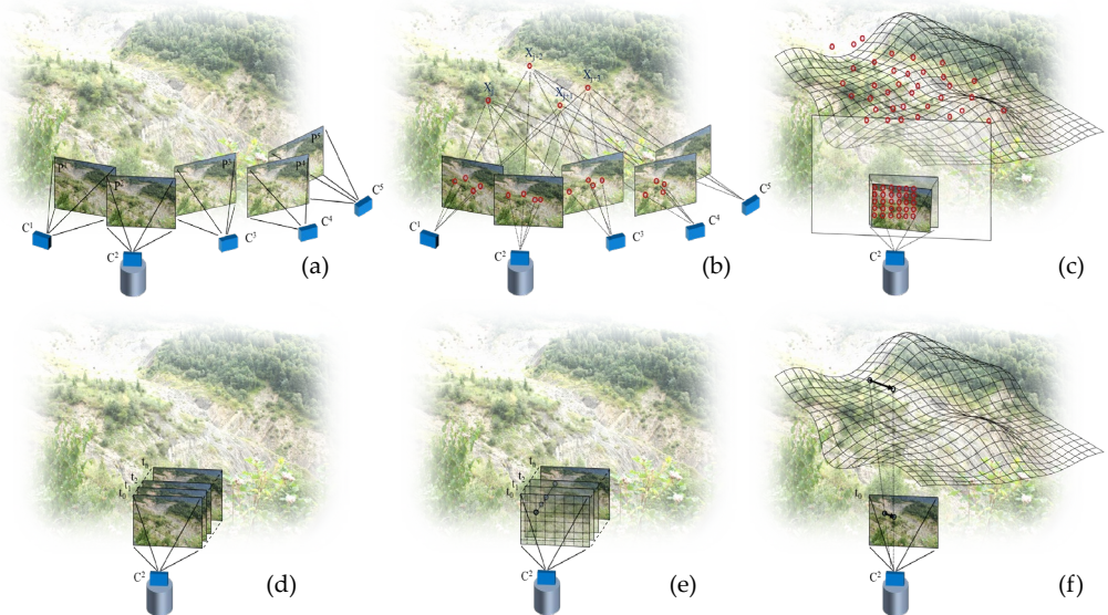
Figure 3. DIPHORM photo-taking, calibration, and processing workflow: (a) Image acquisition from multiple views (including fixed view C^2 ); (b) feature detection, matching of key points, and bundle adjustment for intrinsic parameters and camera pose estimation; (c) image undistortion and calculation of the depth map of the scene based on the dense point cloud previously obtained or with an external registered point cloud (e.g., laser scanner point cloud); (d) collection of time-lapse images from position C^2 ; (e) digital image correlation (NCC metric) applied to a grid of patches on the images; and (f) 3D projection of the 2D displacement on the depth map of the scene. C^1, C^2, \dots, C^5 and P^1, P^2, \dots, P^5 refer to the camera positions and the corresponding photos in the calibration phase. X_i refer to the key points used for matching and t_0, t_1, \dots, t_n to the time steps of the image sequence.
