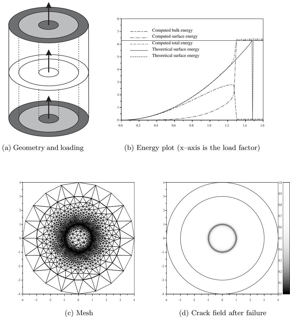
Figure 1: Tearing of a reinforcement, first method
