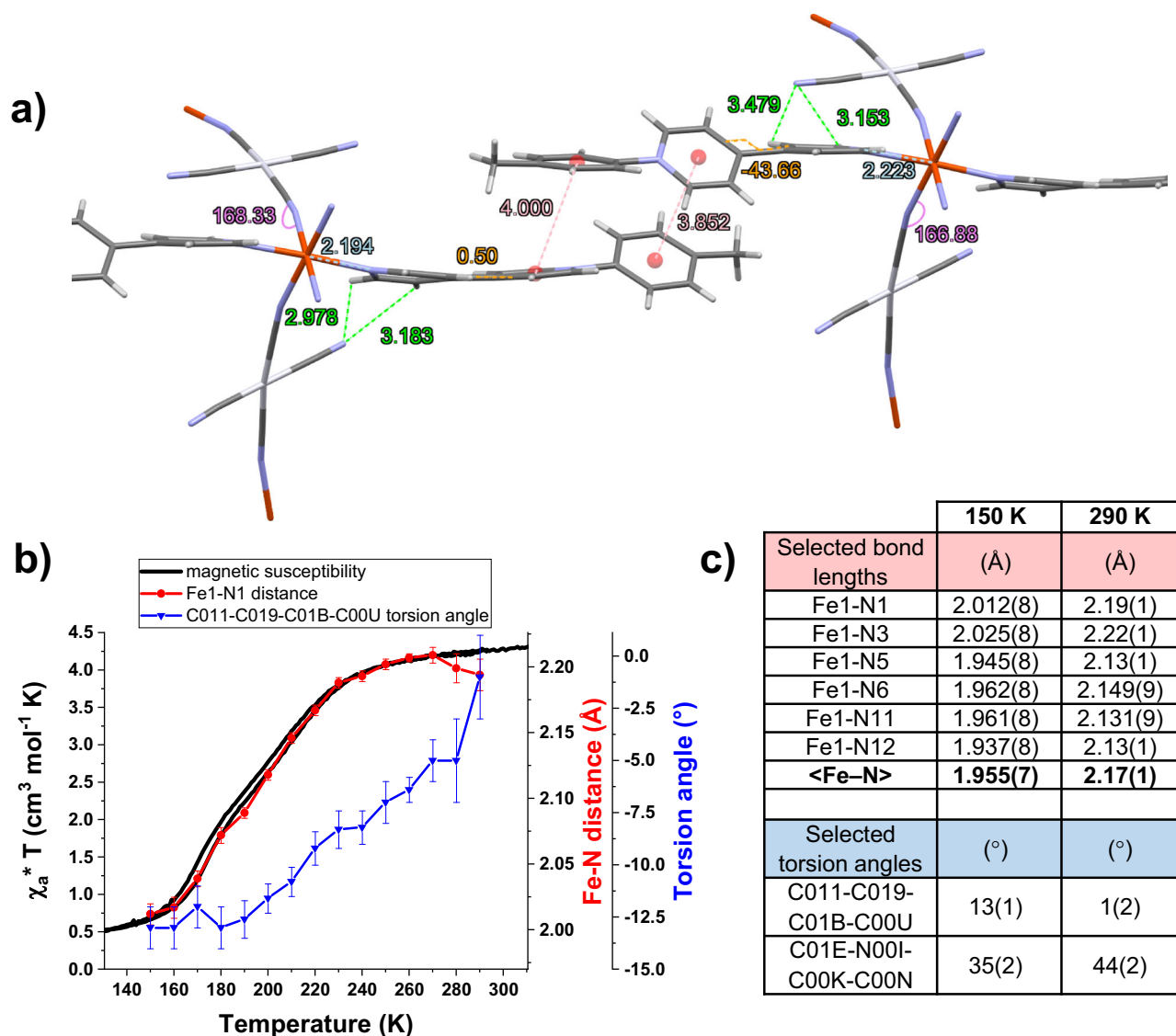
Fig. 9 | In-detail crystallographic analysis of compound 1b . a side view of two stacked units of 1b at 290 K, indicating where interactions and structural changes are observed in temperature. Fe-N distances are marked in light blue, the Fe-N-C angle in purple, the \pi - \pi stacking and bipyridinium-NC distances in red and green, respectively, and torsion angles in orange. Water molecules are omitted for clarity.
