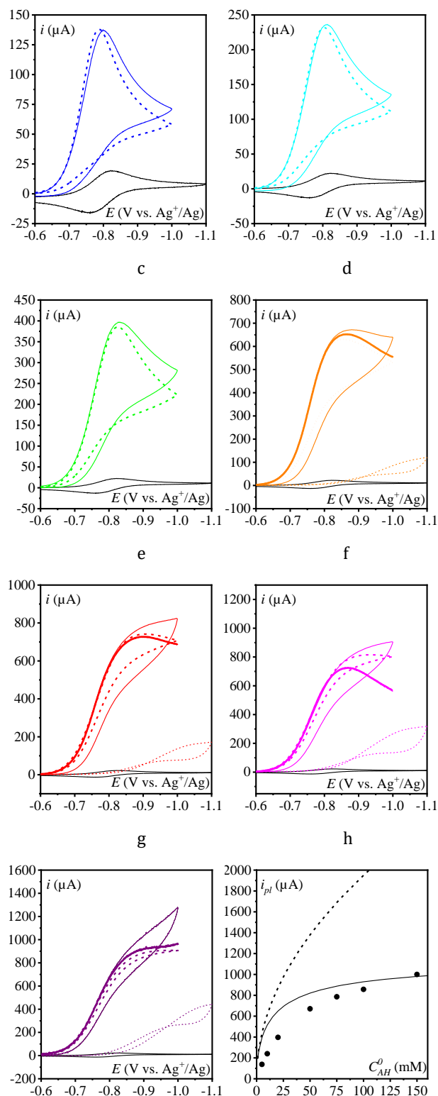
Figure 10. CVs of [\text{Co}^{\text{II}}(\text{CR14})]^{2+} 1 mM in the absence (black) and in the presence (full thin lines in a to h) of 5 (blue), 10 (light blue), 20 (green), 50 (orange), 75 (red), 100 (magenta) and 150 (purple) mM of p -cyanoanilinium acid. From (a) to (h): dashed lines are simulated CVs (see text and SI). From (d) to (g): dotted lines are CVs of the acid alone and thick full lines are forward CV scans obtained after subtraction of the current of the acid alone from the current obtained in the presence of the catalyst.
