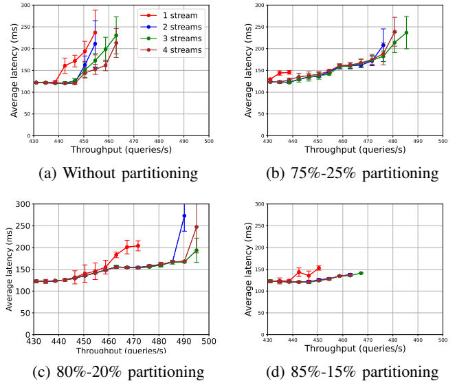
Fig. 9: Executing Nfnet with different partitioning loads and running on multiple streams with a batch size of 27
