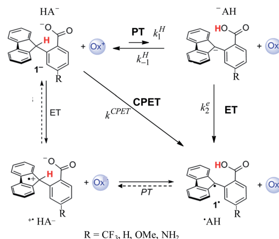
Scheme 1 PCET mechanisms.
