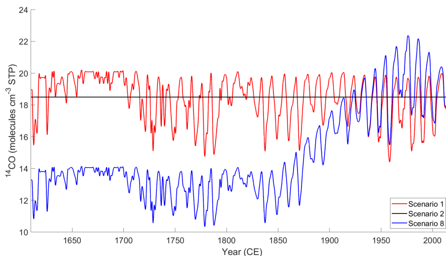
Figure 5. Paleoatmospheric [ ^{14}\text{C} ] scenarios. Visualization of some of the paleoatmospheric ^{14}\text{C} history scenarios used in constraining muogenic ^{14}\text{C} production tuning factors f_{\mu-} and f_{\mu f} . Scenario names in the figure caption correspond to the list in Sect. 4.3.2.
