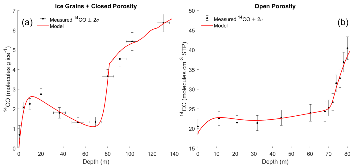
Figure 3. ^{14}\text{CO} measurements at Summit. The ^{14}\text{CO} measured at Summit in ice grains + closed porosity (a) and in open porosity (firn air) (b), together with an example of our firn model fit to the data. Measured values are after all corrections (Table S4).
