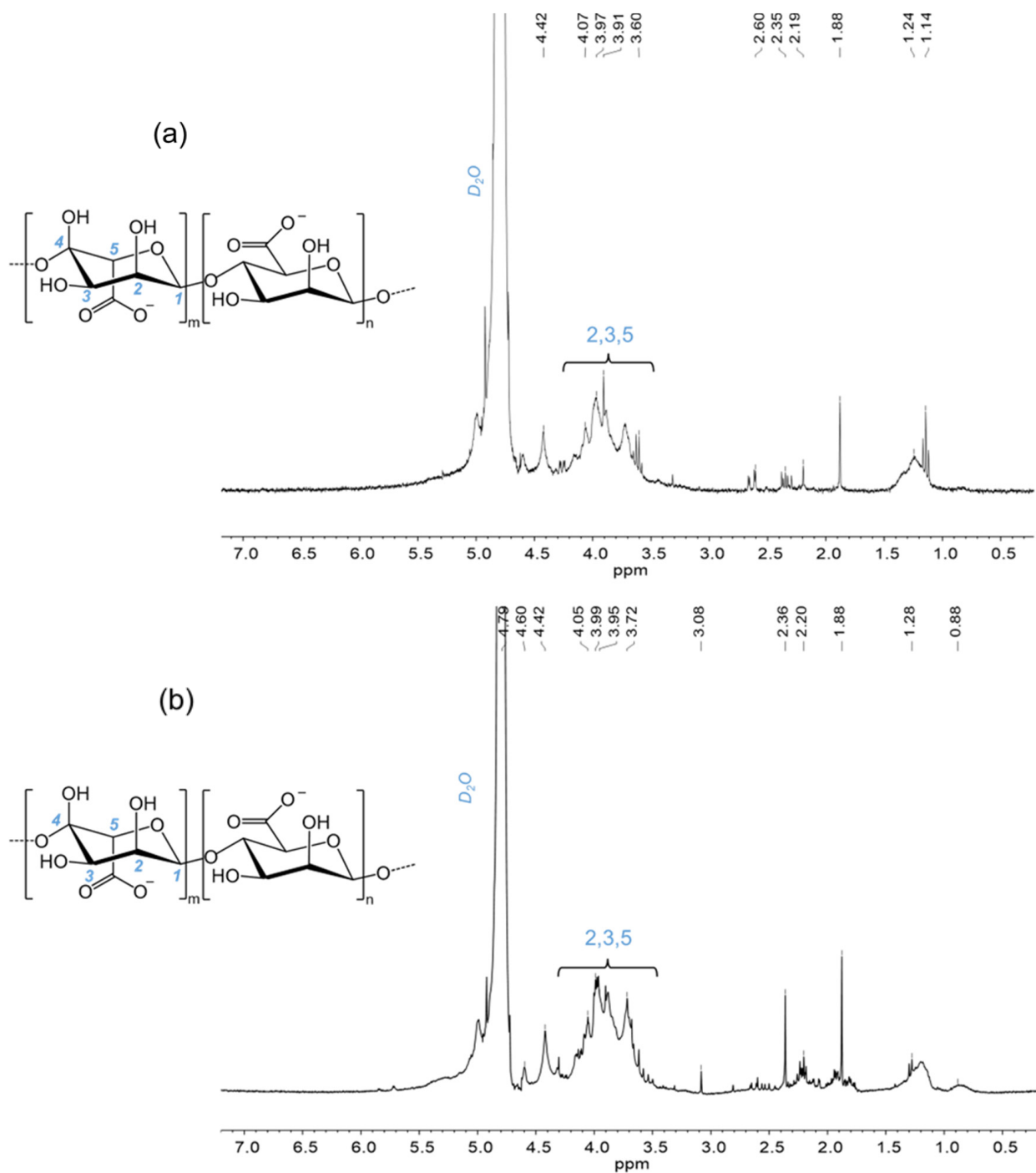
Figure 6. 1 H NMR spectra of sodium alginate samples in D 2 O obtained from (a) protocol 3 and (b) protocol 4.
