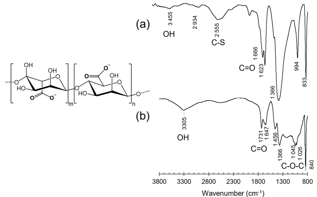
Figure 4. Infrared spectra of alginate samples obtained from (a) protocol 3 and (b) protocol 4.
