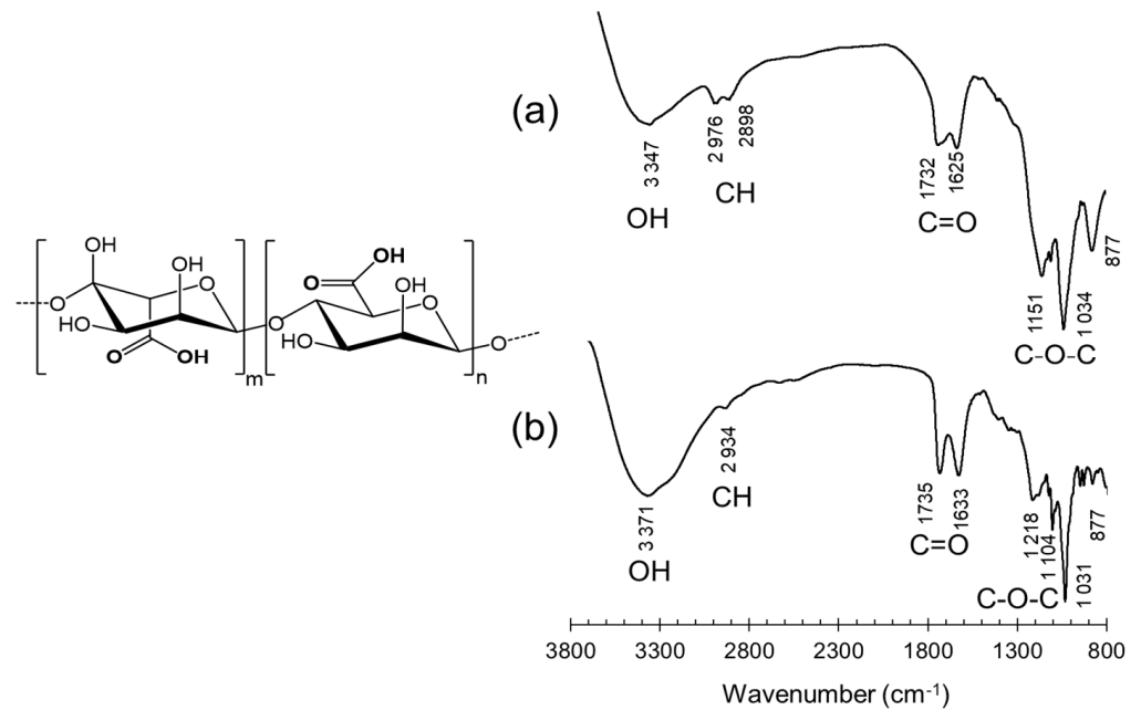
Figure 3. Infrared spectra of alginate acid obtained from (a) protocol 1 and (b) protocol 2.
