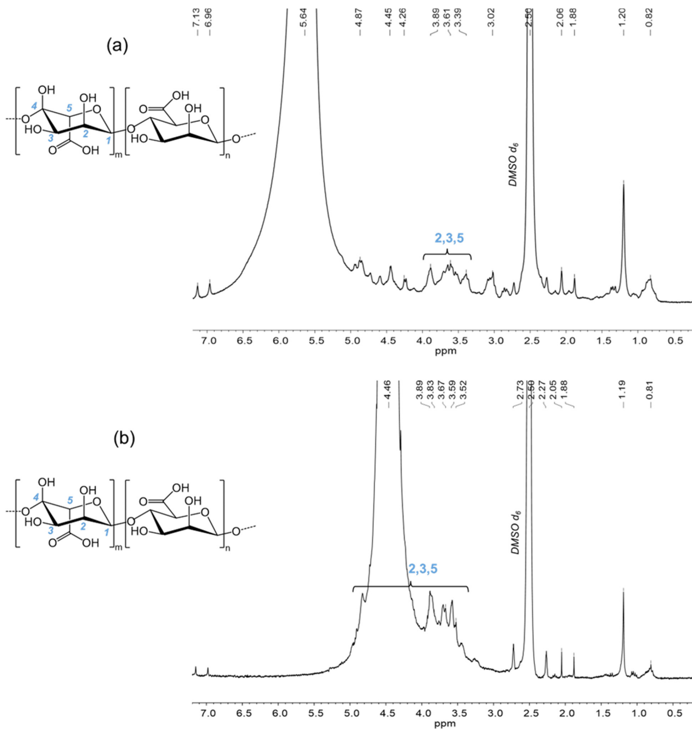
Figure 5. 1 H NMR spectra of alginic acid samples in DMSO d 6 obtained from (a) protocol 1 and (b) protocol 2.
