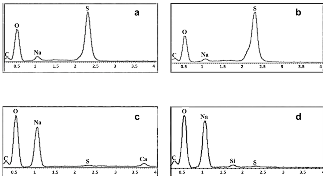
Figure 8. EDX of alginic acid (a,b) and sodium alginate (c,d).
