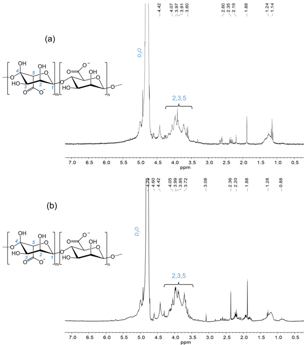
Figure 6. ^1\text{H} NMR spectra of sodium alginate samples in \text{D}_2\text{O} obtained from (a) protocol 3 and (b) protocol 4.
