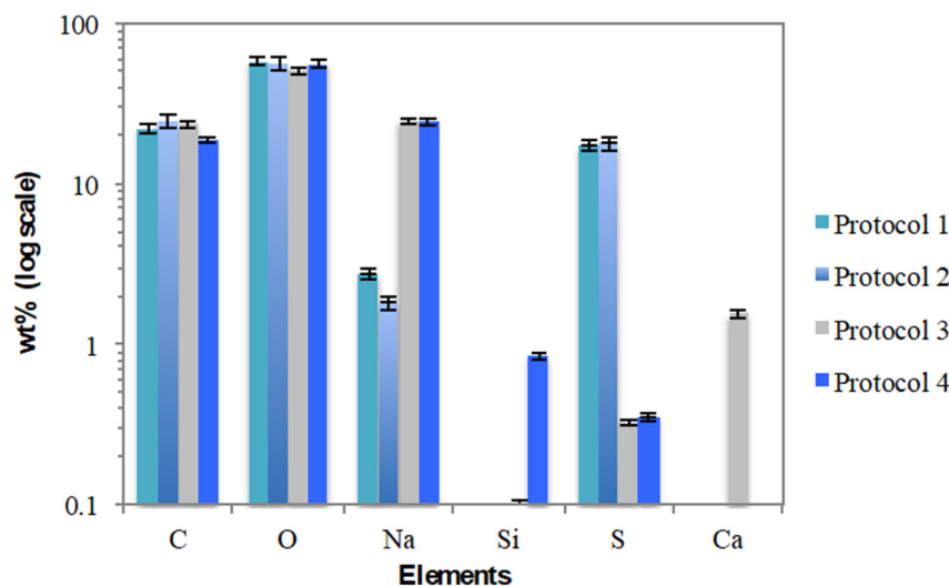
Figure 9. Elemental composition of samples 1 to 4 of alginic acid (protocols 1 and 2) and sodium alginate (protocols 3 and 4) determined via EDX measurements. Analysis shows error bars with \pm S.D. from the mean ( n = 3 ).
