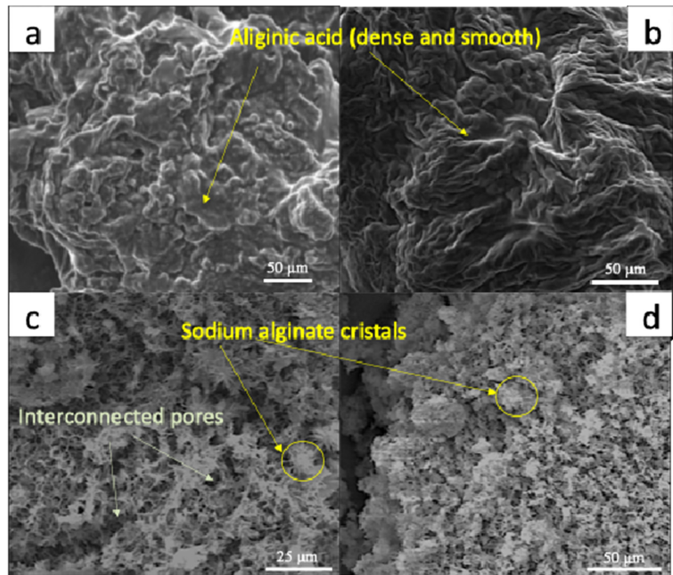
Figure 7. SEM micrographs of alginic acid extracted from (a) protocol 1 and (b) protocol 2, and alginate extracted from (c) protocol 3 and (d) protocol 4.
