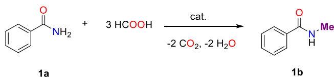
Scheme 1. N-methylation of benzamide ( 1a ) with formic acid.
