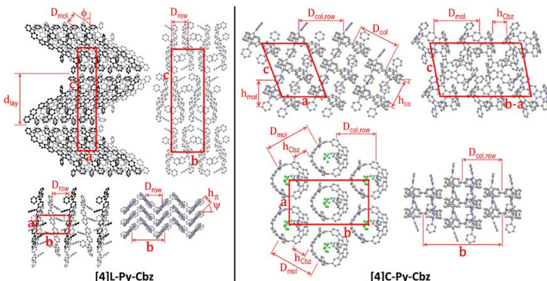
Figure 3. Left part: views of the single-crystal structure of [4]L-Py-Cbz , from left to right and top to bottom, views along the b -axis (molecular slices in the foreground at y = 0.0 , in the background and drawn in black at y = 0.5 ), the a -axis and the c -axis (molecular slice at z = 0 ; molecules in the foreground at x = 0.0 , in the midground and drawn in dark grey at x = 0.5 , in the background and drawn in black at x = 1.0 ), and view along the molecular axes (molecular slice at z = 0 ). Right part: views of the single-crystal structure of [4]C-Py-Cbz , from left to right and top to bottom, views along the b -axis (molecular slices with centroids at y = 0.0 and y = 0.2 ), along the normal to the (\mathbf{b}-\mathbf{a}) \times \mathbf{c} diagonal plane (molecular slice at y = x ) and along the normal to \mathbf{a} \times \mathbf{b} plane (molecular slice at z = 0.0 ), and view in the molecular loop plane (molecular slice at z = 0.0 ). For sake of clarity, hydrogens are not shown and the solvent molecules co-crystallized with [4]C-Py-Cbz are only displayed for one view. The definition and value of the characteristic distances are given in Table 2.
