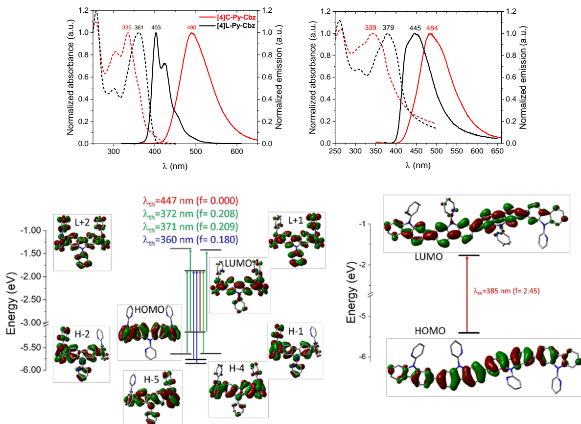
Figure 4. [4]C-Py-Cbz and [4]L-Py-Cbz . Top: Absorption (dash) and emission (full) spectra in cyclohexane (left, \lambda_{\text{exc}} = 310 nm for [4]L-Py-Cbz and \lambda_{\text{exc}} = 350 nm for [4]C-Py-Cbz ) and in thin film (middle, \lambda_{\text{exc}} = 360 nm for [4]L-Py-Cbz and \lambda_{\text{exc}} = 340 nm for [4]C-Py-Cbz ). Normalized emission and delayed emission at 77 K, in 2-Me-THF, of [4]C-Py-Cbz (red lines, \lambda_{\text{exc}} = 400 nm for both) and of [4]L-Py-Cbz (black lines, \lambda_{\text{exc}} = 350 and 400 nm respectively). Bottom: Representation of the energy levels and the main molecular orbitals involved in the electronic transitions obtained by TD-DFT, B3LYP/6-311+G(d,p), shown with an isovalue of 0.02 [ebohr -3 ] 1/2 .
