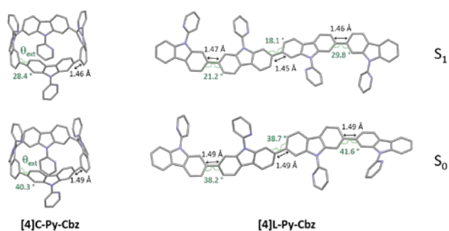
Figure 5. Optimized geometries (B3LYP/6-31+g(d)): S_0 (ground state, bottom) and S_1 (first singlet excited state, top) of [4]C-Py-Cbz (left) and [4]L-Py-Cbz (right). On each structure, in the S_0 and S_1 states, the modelized mean torsion angle \theta_{\text{ext}} between the carbazoles and the length of the C-C bond linking two carbazoles are presented.
