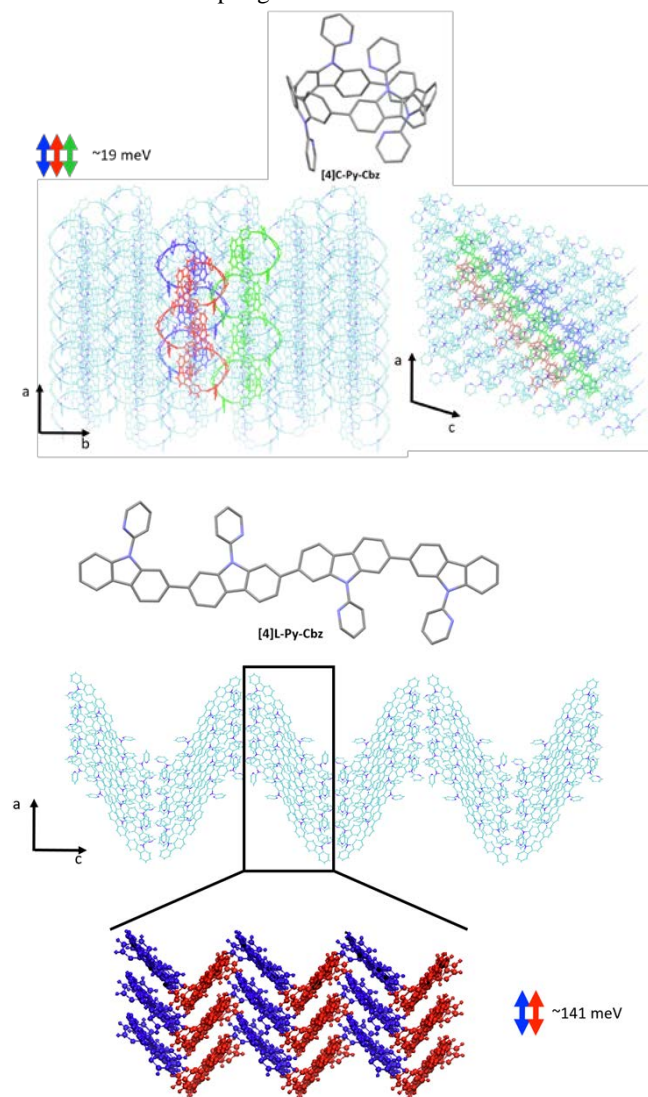
Figure 7. Transport direction yielding the highest transfer integrals in the crystalline structure of [4]C-Py-Cbz (top) and [4]L-Py-Cbz (bottom).
