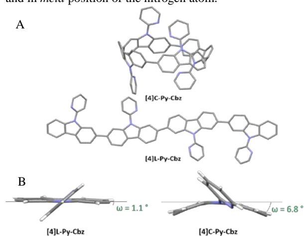
Figure 2. A. Single-crystal structures of [4]C-Py-Cbz (Top, CCDC n° 2265379) and [4]L-Py-Cbz (Bottom, CCDC n° 2325120). B. Representation of the displacement angle \omega showing the deformation of the carbazole unit
