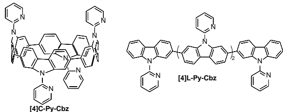
Figure 1. Molecular structures of tetracarbazole oligomers: cyclic [4]C-Py-Cbz (Left) and acyclic [4]L-Py-Cbz (Right).
