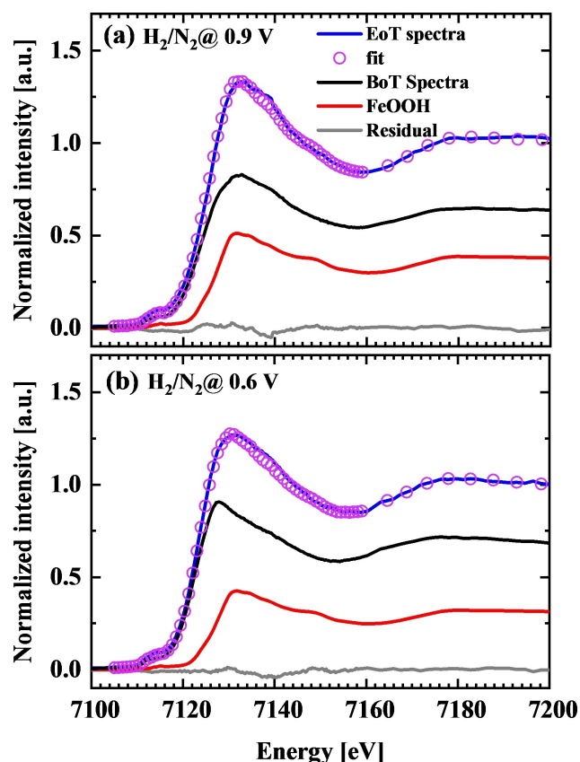
Figure 8. Results of the LCF on the EoT spectra of the H_2/O_2@0.8 V test (blue, as in Figure 7) recorded under H_2/N_2 at 0.9 V (a) and 0.6 V (b), using a combination of the spectrum at BoT (black line, as in Figure 7) and of the spectrum of FeOOH (red line). The purple circles represent the LCF curve, while the gray line is the residual signal after subtracting the LCF from the measured spectrum.
