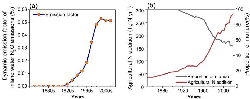
Fig. 5 | Global mean emission factors of N 2 O emissions from inland waters. a Dynamics of mean global emission factors for inland water N 2 O emissions. b Dynamic amount of agricultural nitrogen addition and the proportion of manure in agricultural nitrogen addition.
