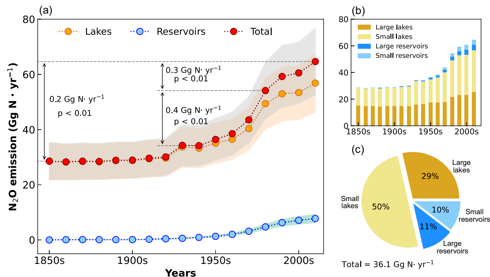
Fig. 1 | Changes in N 2 O emissions from global lakes and reservoirs since the pre-industrial period. a Total N 2 O emissions from global lakes and reservoirs (red dotted line) and N 2 O emissions from global lakes (orange dotted line) and global reservoirs (blue dotted line) during the 1850s-2010s; the orange, blue, and gray bands represent the uncertainty (mean \pm standard deviation of the annual average) of N 2 O emissions. b N 2 O emissions from different lentic systems. c The relative contribution of different lentic systems to overall increase in global N 2 O emissions from lakes and reservoirs during 1850s-2010s.
