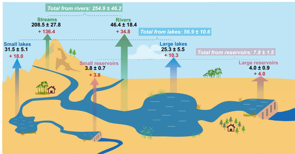
Fig. 4 | Global inland water N 2 O emissions for the 2010s. The colored arrows represent N 2 O emissions as follows: green, emissions from streams and rivers; blue, emissions from small and large lakes; pink, emissions from small and large reservoirs. The colored numbers represent N 2 O fluxes as follows: bold black numbers, the emissions in the 2010s; bold red numbers, the increased emissions during the
