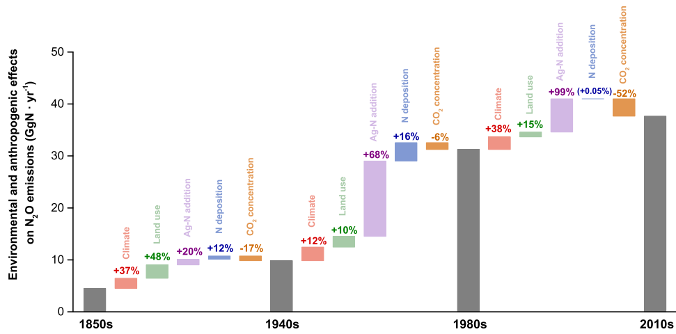
Fig. 3 | The relative contributions of environmental and anthropogenic factors to N 2 O emission changes from global lakes and reservoirs over different time periods. The gray bars show mean decadal N 2 O emissions from global lakes and reservoirs induced by five forcing factors. The colored bars and their percentages
