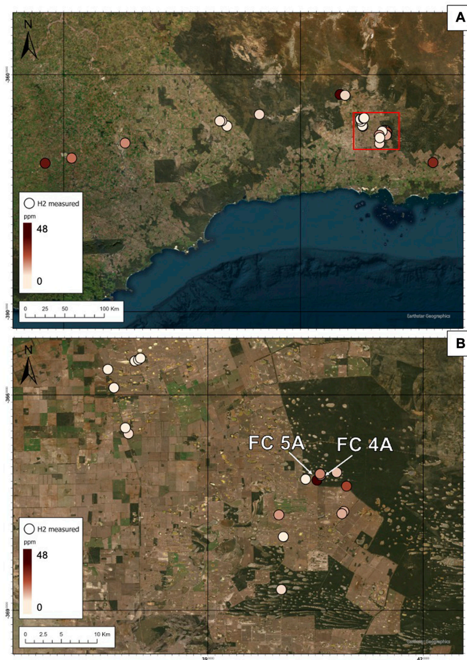
FIGURE 8 (A) Hydrogen measurements from several field missions over southern Western Australia. The red square indicates the studied area in this paper (B) Hydrogen measurements in the studied area. FC 5A and 4A are the monitored features. The measurements in the northern western part are from another field campaign (Images Earthstar Geographics).
