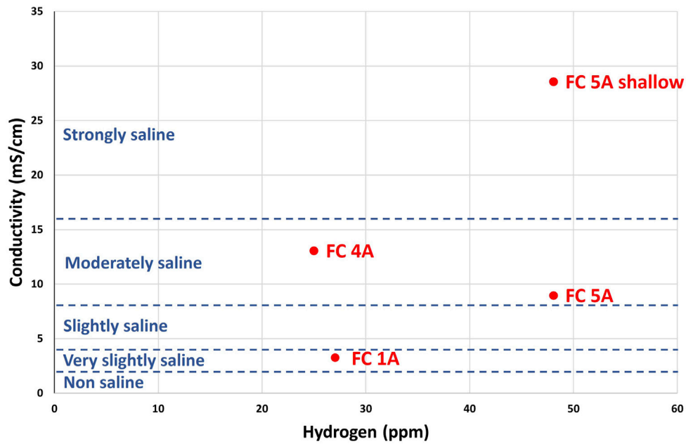
FIGURE 11 Electrical conductivity of the samples compared to the maximum amount of hydrogen measured at the feature. FC 5A shallow represents the sample from the first 10 cm. The saline classification is as defined in the U.S. National Soil Survey Handbook.
