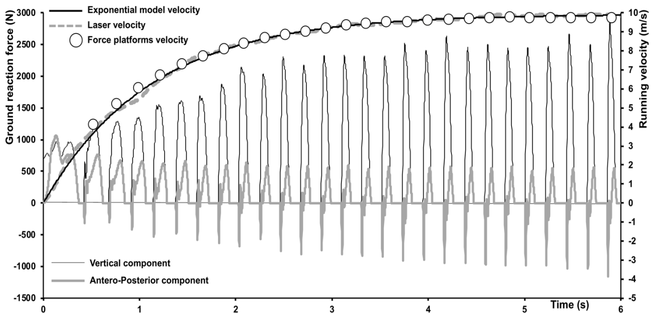
Fig. 1. Typical example of raw data of running velocity, vertical and antero-posterior components of the ground reaction force during the first 6 seconds of a 60-m sprint acceleration. Circles indicate step-averaged values of running velocity, over the corresponding step, after the starting-block push-off. The running velocity traces obtained from the laser system and the associated exponential fitting are almost overlapping.
