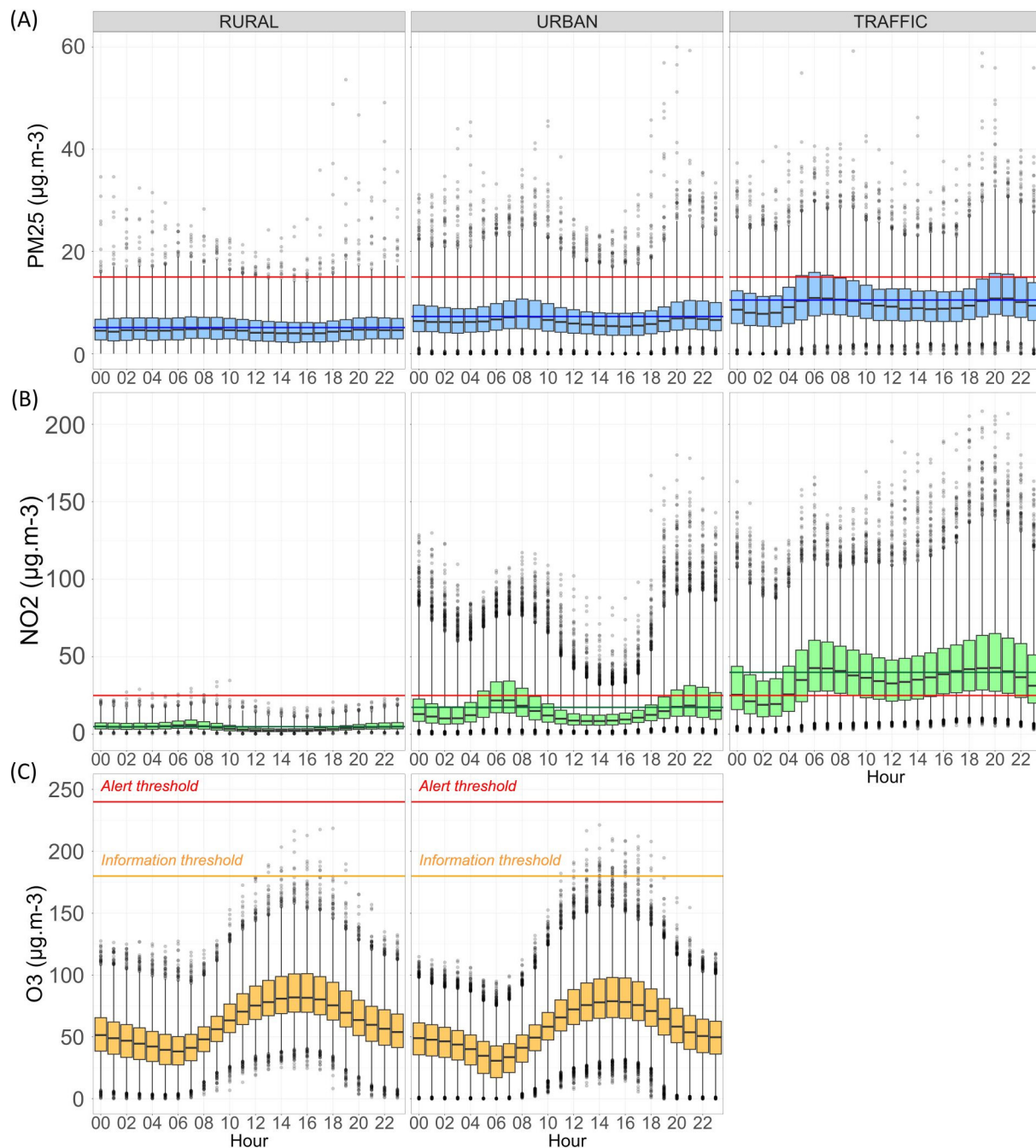
Figure 1 Hourly diurnal cycle of (A) particulate matter ( PM_{2.5} ), (B) nitrogen dioxide ( NO_2 ) and (C) ozone ( O_3 ) concentrations measured in the Paris area at traffic, urban and rural sites of the Airparif air quality network for the summer months (July–September) of the period 2020–2023. UTC: coordinated universal time. The distributions of hourly values are represented by boxplots indicating the median, interquartile 25–75, inter-percentile 0.01–0.99. The circles are the outliers, that is, the 1% lowest and highest values. (A) The blue line indicates the daily global mean and the red line indicates the daily WHO recommended level ( 15 \mu\text{g}/\text{m}^3 ) not to be exceeded more than 3–4 days per year for PM_{2.5} . To keep the value scales homogeneous between the figures, the 16 highest values are not present in the figure with a maximum value of 107 \mu\text{g}/\text{m}^3 ; (B) horizontal green line indicates the daily global mean, and the red line indicates the daily WHO recommended level not to be exceeded of 25 \mu\text{g}/\text{m}^3 . To keep the value scales homogeneous between the figures, the nine highest values (all at traffic station) are not present in the figure with a maximum value of 323 \mu\text{g}/\text{m}^3 ; (C) horizontal red line indicates the French information (hourly mean 180 \mu\text{g}/\text{m}^3 ) and alert (hourly mean 240 \mu\text{g}/\text{m}^3 ) thresholds.
