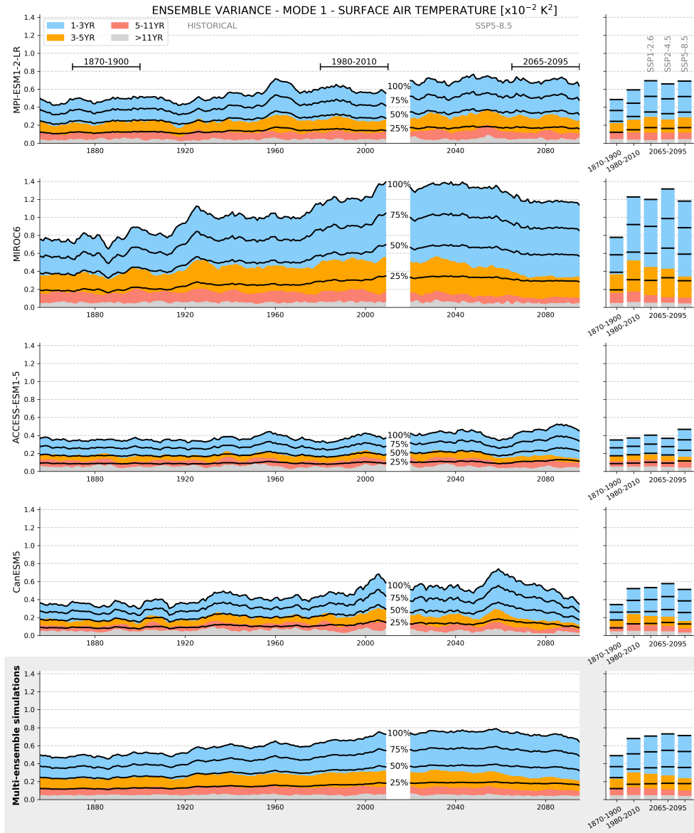
FIG. 9: Ensemble variance of globally-averaged Surface Air Temperature explained by the first EOF mode. Each row corresponds to a given model, except the last one which is the concatenation of all of them. The rows present the ensemble variance over the historical and projection (SSP5-8.5) periods. Similarly to Fig. 1, the colors represent the contribution of the various frequency of variability to the variance and the right panels gathers information for three climatic periods (1870-1900, 1980-2010 and 2065-2095) and for the three investigated scenarios for the last period (2065-2095). The black lines represent the quarters of the total variance.
