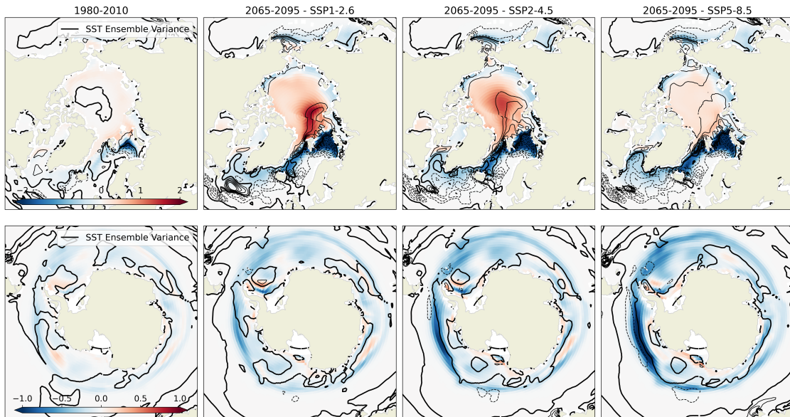
FIG. 7: Comparison between Sea-ice Concentration and Sea Surface Temperature ensemble variance changes. Similarly to Fig. 5, colors represent the changes of sea-ice concentration ensemble variance (in %) compared to the early historical reference (1870-1900). Contours represent the changes of sea surface temperature ensemble variance (in K^2 ) compared to the early historical reference. The thick lines represent the zero contour and the thin solid and dashed lines represent respectively the positive (increase) and negative (decrease) contours. The first line shows the results around the North Pole, the contours are plotted from -1 to 1 K^2 every 0.2 K^2 . The variances are smaller around the South Pole, therefore the colormap and contours values are reduced by half.
