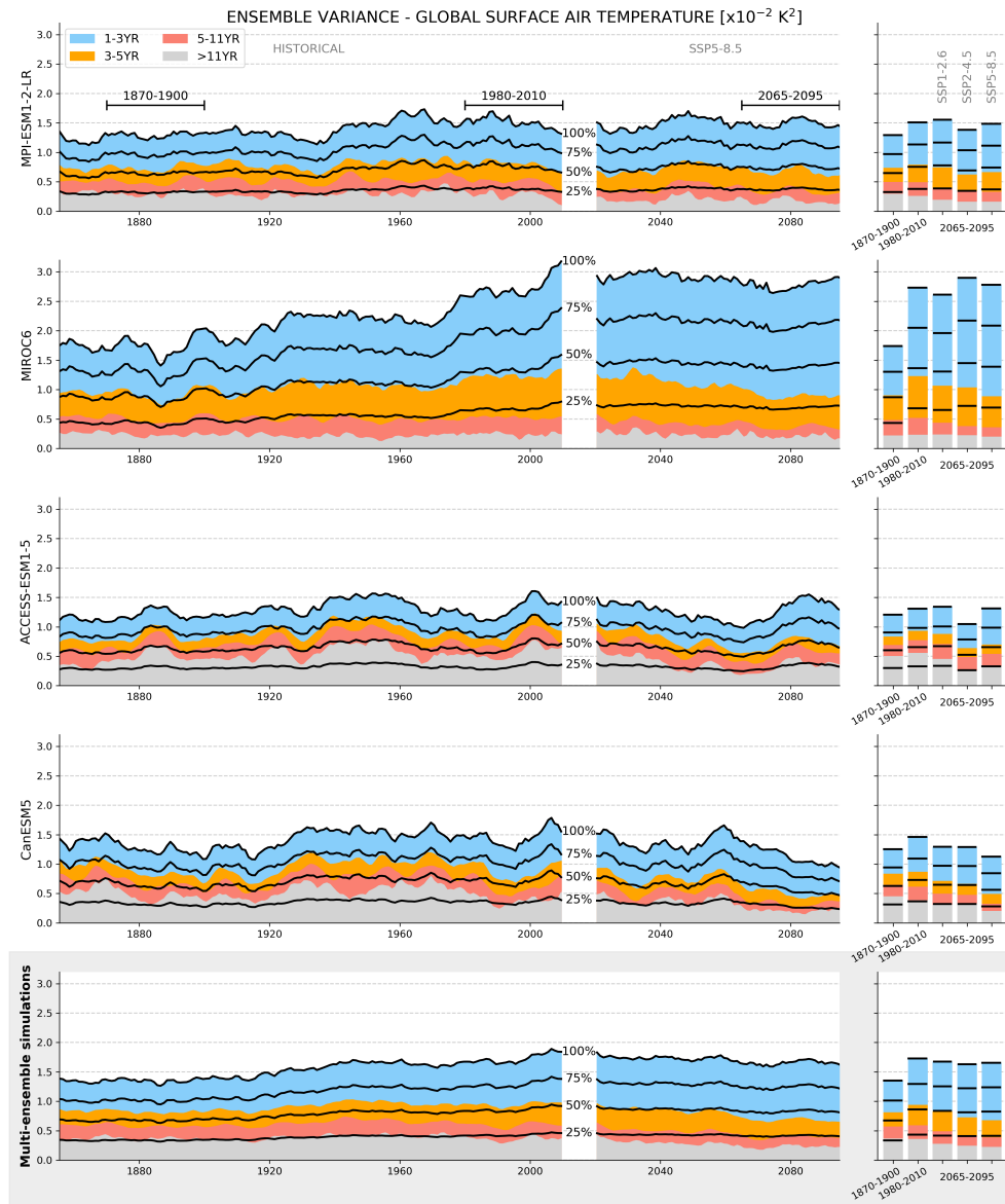
FIG. 1: Ensemble variance of globally-averaged surface air temperature. The four first rows show the ensemble variance for four different models: MPI-ESM1-2-LR, MIROC6, ACCESS-ESM1-5 and CanESM5. The last row presents the variance computed from a multi-ensemble constructed from the concatenation of the four previous models. The left panels presents the yearly results for the historical and projected period with the Fossil-fueled Development scenario (SSP5-8.5). The colors represent the contribution of the various frequency bands to the total variance: blue for the variability with a period band of 1-3 yr, orange for 3-5 yr, red for 5-11 yr, and grey for periods longer than 11 yr. The bands are obtained from a temporal filtering of temperature at the given period and all the bands of variance are finally filtered to be consistent with the 11 yr period. The right panels present the results for a given climatic period (averaged over 30 yr): early historical (1870-1900), end of historical (1980-2010) and end of projections (2065-2095) for three shared socioeconomic pathways, Sustainability (SSP1-2.6), Middle of the Road (SSP2-4.5) and Fossil-fueled Development (SSP5-8.5). The black lines represent the quarters of the total variance.
