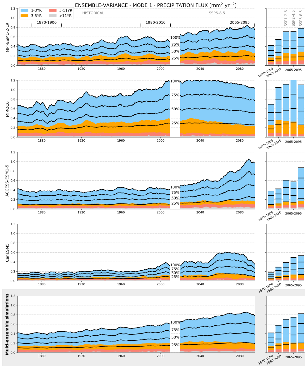
FIG. 10: Ensemble variance of globally-averaged precipitation flux explained by the first EOF mode. As in Fig. 9 but for precipitation.
