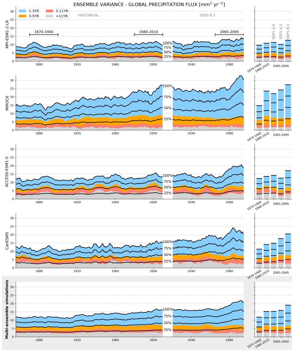
FIG. 2: Ensemble variance of globally-averaged precipitation. As Fig. 1 but for precipitation.
