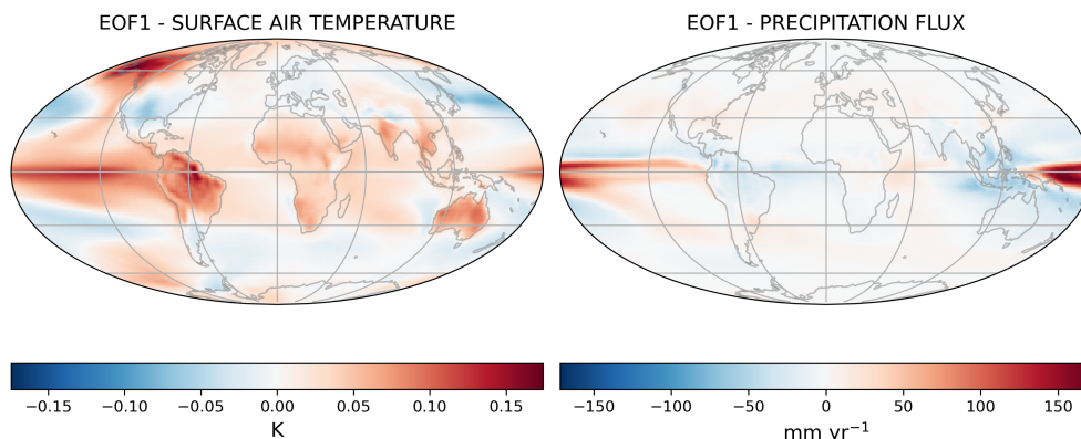
FIG. 8: First Empirical Orthogonal Functions from a Singular Value Decomposition of SAT and Precipitation. The first EOF modes for (left) Surface Air Temperature and (right) Precipitation multiplied by the standard deviation of the first principal component. The first mode of SAT explains 15% of the variance of the entire data set, the second mode explains only 6%. For precipitation, the first mode explains 24% of the variance and the second mode only 5%.
