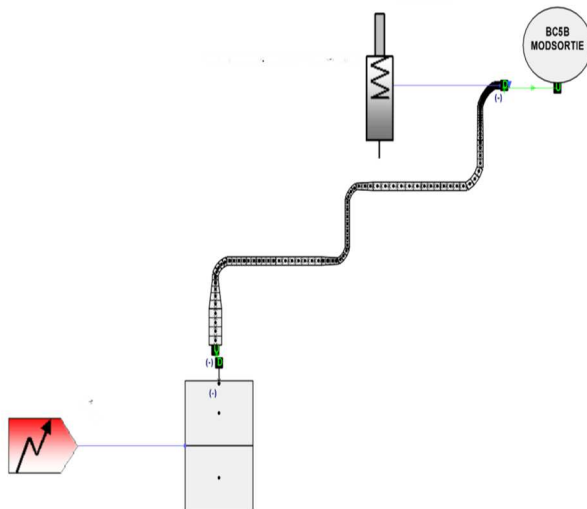
Figure 15 CATHARE-3 model of the Cryostat Soupape experiment
