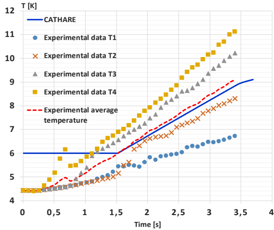
Figure 17 Helium temperature increase in the tank of the Cryostat Soupape
