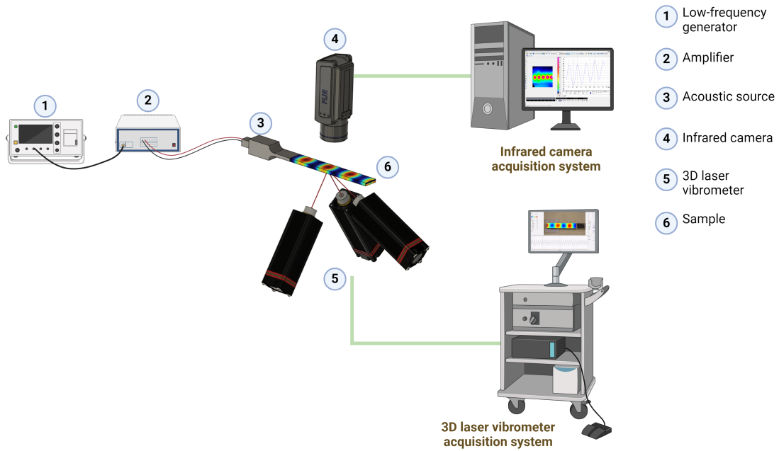
Figure 5: Experimental set-up.
