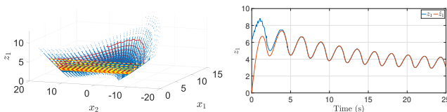
Fig. 1: Left: Data points (x, z_1) in look-up table (blue), and t \mapsto (x(t, j), z_1(t)) along a solution (red-yellow), where z_1(t) is fetched as the closest point in the look-up table; Right: t \mapsto z_1(t) from look-up table obtained from t \mapsto x(t, j) vs. t \mapsto \hat{z}_1(t) solution to observer (19).
