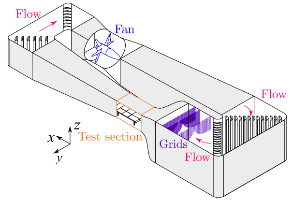
Fig. 5. S620 Wind tunnel schematization. Source: Adapted from Bao (2023).
