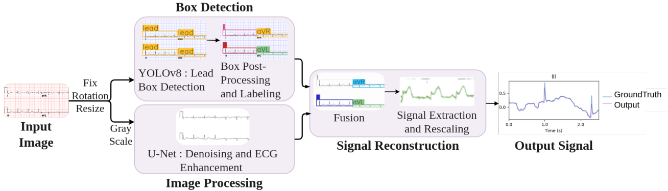
Figure 1. Workflow of YOUR-Lead for a given ECG paper image (we only show part of a 12-lead ECG image for better visualization). The input image passes through two image processing steps to obtain the corresponding binarized clean image and the lead boxes. ECG signals are reconstructed from separate ECG image patches.
