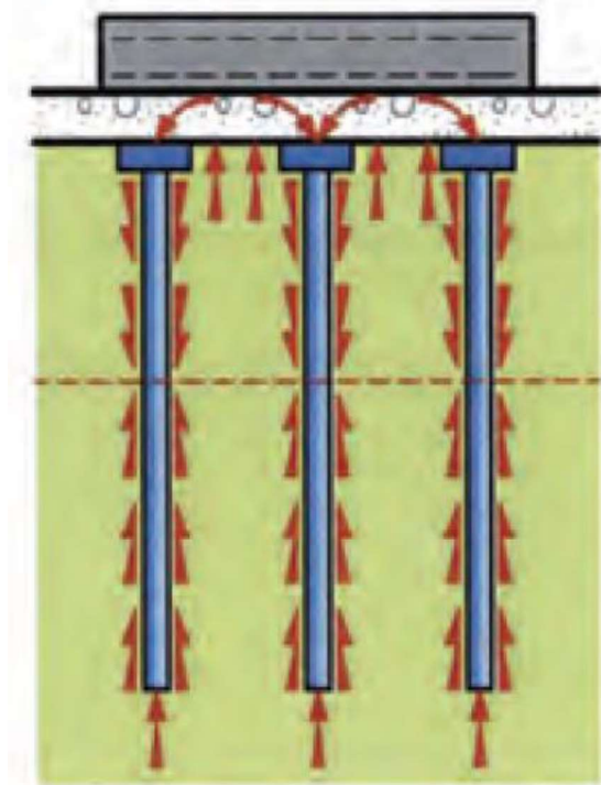
Figure 1. Behaviour of rigid inclusion system (ASIRI, 2012)
