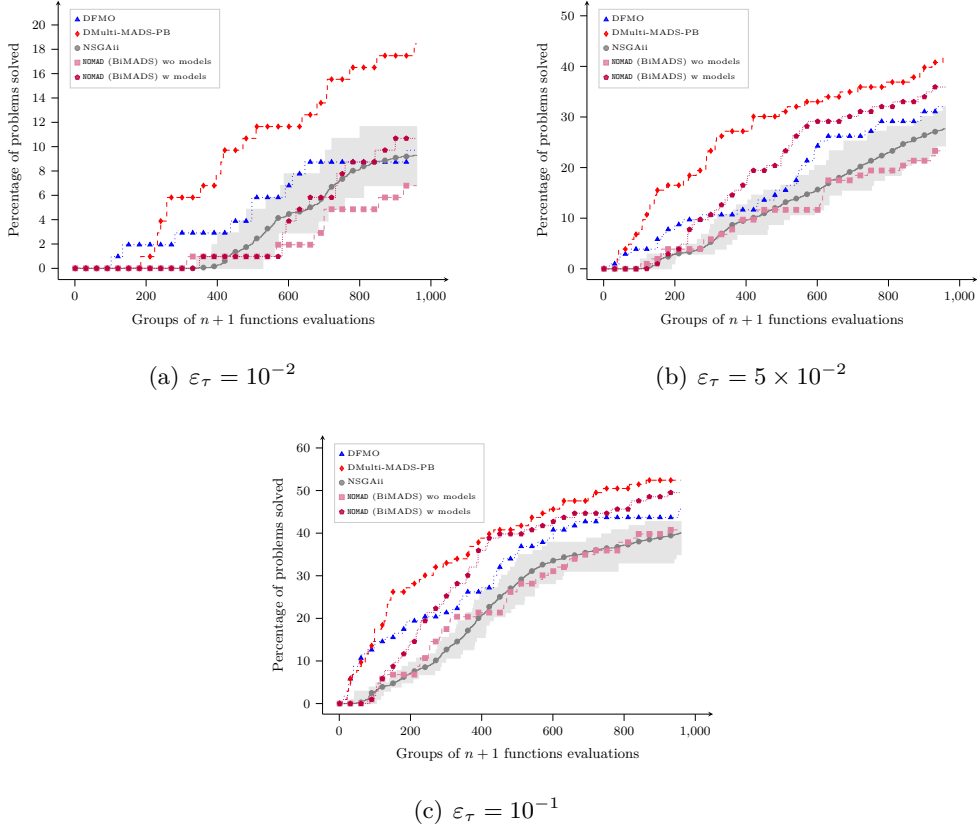
Figure 10: Data profiles using NOMAD (BiMADS), DFMO, DMulti-MADS-PB and NSGA-II obtained on 103 biobjective analytical problems from [46] with 30 different runs of NSGA-II with tolerance \varepsilon_\tau \in \{10^{-2}, 5 \times 10^{-2}, 10^{-1}\} .
