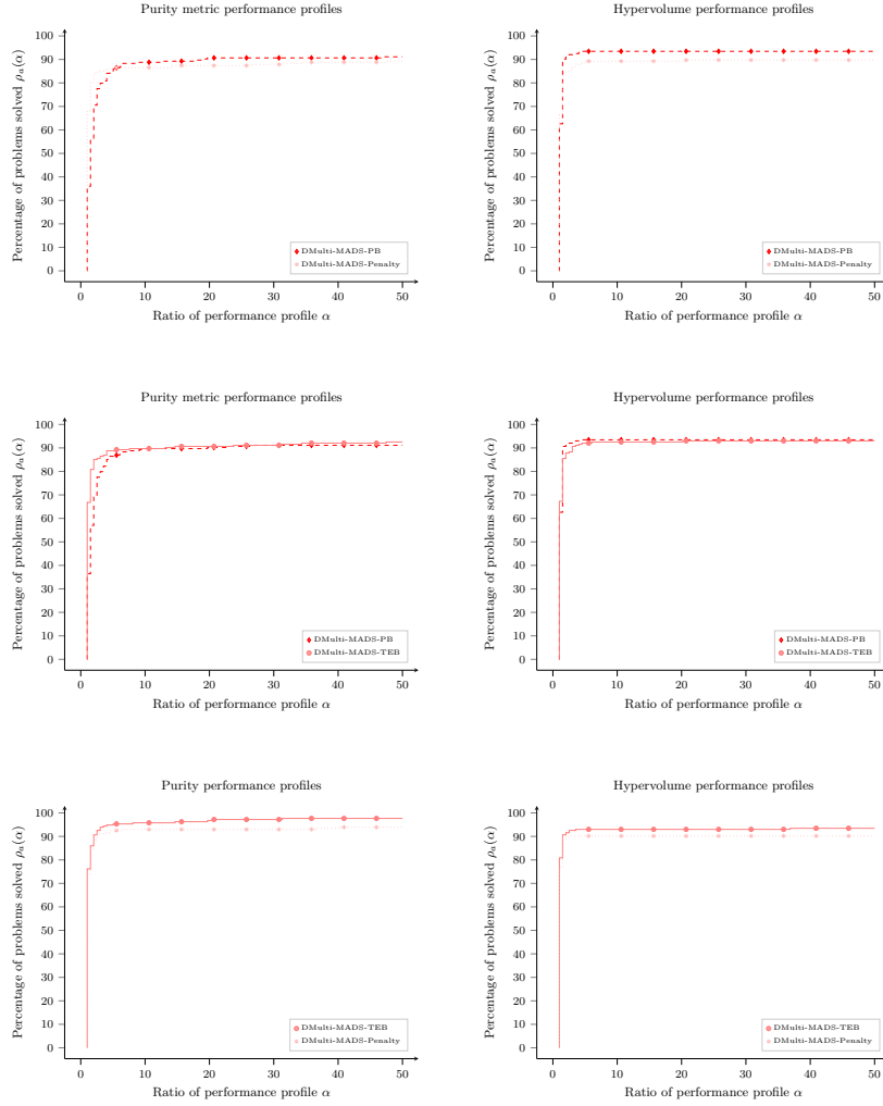
Figure 15: Performance profiles using purity metric and hypervolume with DMulti-MADS-PB, DMulti-MADS-TEB and DMulti-MADS-Penalty obtained from 214 multiobjective analytical optimization problems taken from [46] with a maximal budget of 30,000 function evaluations.
