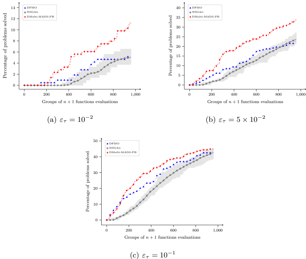
Figure 11: Data profiles using DFMO, DMulti-MADS-PB and NSGA-II obtained on 214 multiobjective analytical problems from [46] with 30 different runs of NSGA-II with tolerance \varepsilon_{\tau} \in \{10^{-2}, 5 \times 10^{-2}, 10^{-1}\} .
