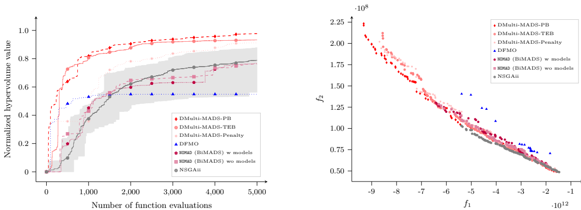
Figure 12: (a) On the left, convergence profiles for the SOLAR8 problem using DFMO, DMulti-MADS, NOMAD (BiMADS) and NSGA-II with 10 different runs of NSGA-II for a maximal budget of 5,000 evaluations. (b) On the right, Pareto front approximations obtained at the end of the resolution of SOLAR8 for DFMO, DMulti-MADS, NOMAD (BiMADS) and an instance of NSGA-II in the objective space.
