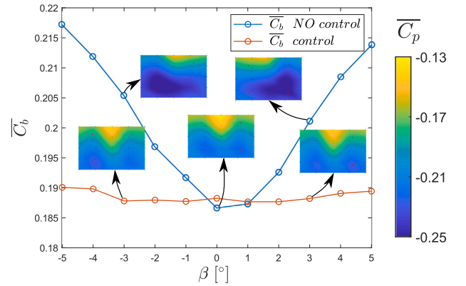
Fig. 9. Mean value of the base pressure C_b versus \beta with (orange line) and without (blue line) control. The standard deviation of C_b is about 2% of \overline{C}_b in all depicted cases.
