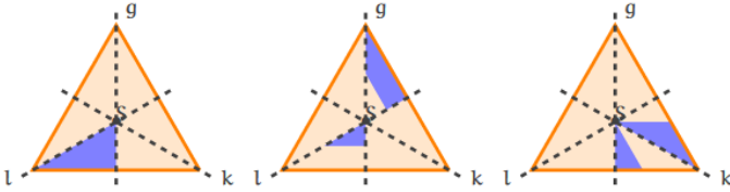
Figure 2. – Visualization of different fundamental domains of the equilateral triangle from Figure 1. In each case, there is exactly one point from the orbit of each point in the subsets marked in blue.
