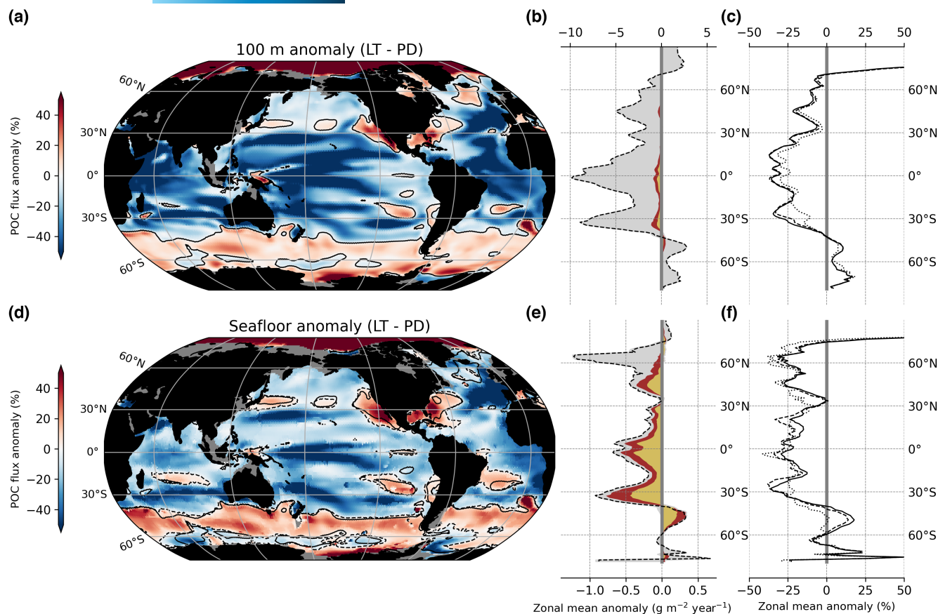
FIGURE 6 Global and zonally averaged POC flux anomalies for LT (2081–2100) versus PD (1995–2014) for the PISCES-FFGM RCP8.5 simulation. Anomaly (%) computed (a) at 100 m and (d) at the seafloor (>1000 m). Black lines indicate the limits between positive and negative anomalies at 100 m (plain) and at the seafloor (>1000 m, dotted). (b) and (e) Zonal mean absolute anomalies computed (b) at 100 m and (e) at the seafloor ( \text{gC m}^{-2} \text{year}^{-1} ). The dashed line shows the anomaly for total POC. The fill colors show the contribution of the different components of the POC: small and medium particles in gray, GM carcasses and fecal pellets in red, and FFGM carcasses and fecal pellets in yellow. (c) and (f) Zonal mean anomalies (%) at 100 m and at the seafloor, respectively, for the standard PISCES-FFGM run (plain line) and the two sensitivity experiments: PISCES-GM (dashed line), and PISCES-v2 (dotted line).
