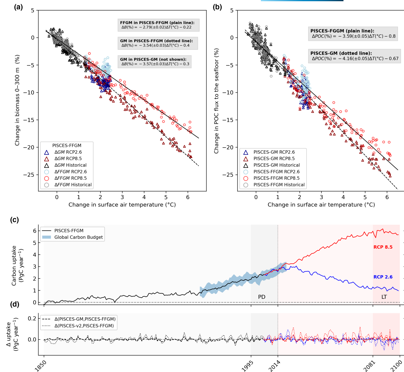
FIGURE 3 Projected changes in macrozooplankton biomass and their impacts on carbon fluxes and carbon uptake under RCP8.5 and RCP2.6 scenarios. (a) Projected trends of PISCES-FFGM upper 300m mean GM and FFGM biomass in relation to global air temperature changes since preindustrial times (1850–1900). Gray boxes show the relationships estimated with linear regression fits. The slope is a proxy for biomass change per degree of warming. (b) Projected trends of PISCES-FFGM and PISCES-GM POC export at the seafloor (>1000m) as a function of global air temperature changes since preindustrial times (1850–1900). Gray boxes show the relationship estimated from linear regression fits. The slope is a proxy of export flux change per degree of warming. (c) Time series of the mean anthropogenic carbon uptake ( \text{PgC year}^{-1} ). Shaded area is the Global Carbon Budget 2021 ocean sink product (uncertainty of \pm 0.4 \text{ PgC year}^{-1} on average) and is estimated from the average of eight global ocean biogeochemistry models (including NEMO-PISCES) and the average of seven ocean f\text{CO}_2 data products (Friedlingstein et al., 2022). PD and LT indicate present-day (1995–2014) and long-term (2081–2100) reference periods. (d) Time series of the annual differences in mean anthropogenic carbon uptake ( \text{PgC year}^{-1} ) for PISCES-v2 and PISCES-GM compared with PISCES-FFGM.
