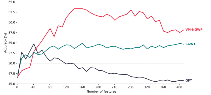
Fig. 2. Comparison of classification accuracies between control and depressed adolescents across increasing numbers of features.
