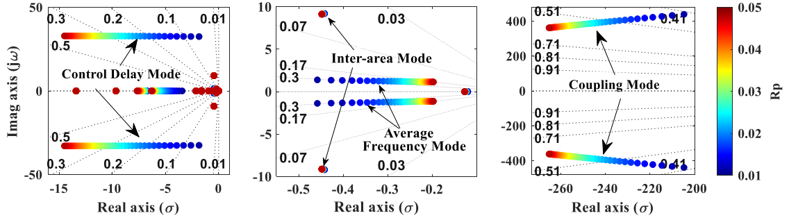
Figure 9: The displacement of the eigenvalues in the complex plane when R_p is varied.
