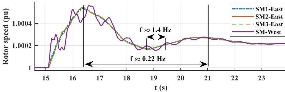
Figure 8: SM's rotor speed after a step change of the inverter's power setpoint of 0.05 pu.
