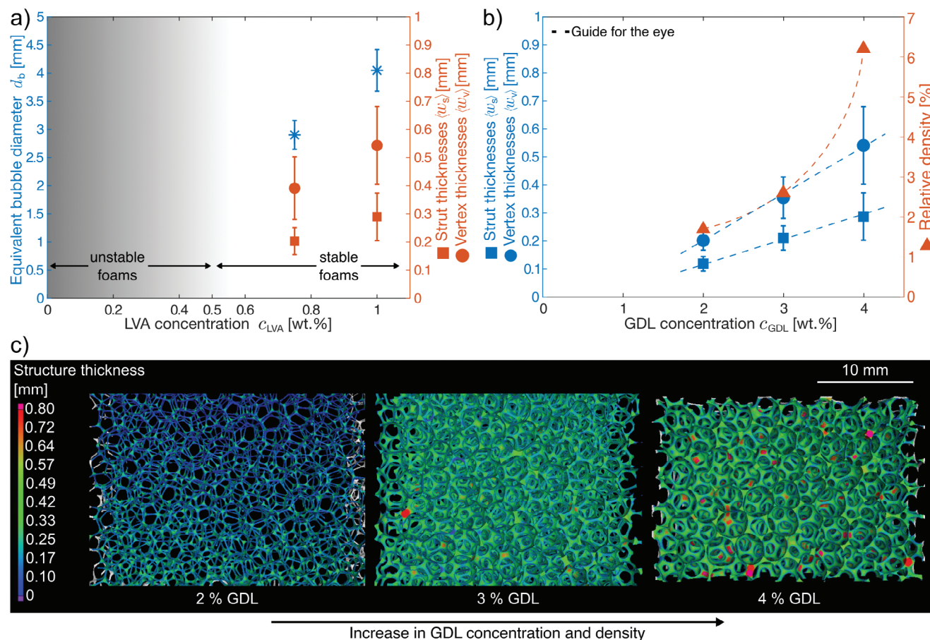
Figure 7. Impact of the formulation on the foam features a) Influence of the LVA concentration: left axis in blue: Equivalent bubble diameters d_b . Right axis in red: Average thickness of struts w_s and vertices w_v over the entire sample. All results are measured with the VG Studio software on LVA foam tomographic scans for different LVA concentrations c_{LVA} (with 0.02 M CaHPO 4 + 2 wt% Disponil + 4 wt% GDL). The error bars correspond to standard deviations of bubble diameters or strut thicknesses, respectively, over the entire sample. A foam with c_{LVA} = 0.5 wt% was tested and found to be unstable. 0.5 wt% of LVA is therefore marked on the graph as the boundary between unstable and stable foams. b) Influence of the GDL concentration: left axis in blue: Average thickness of struts \langle w_s \rangle and vertices \langle w_v \rangle over the entire sample. All results are measured with the VG Studio software on LVA foam images for different GDL concentrations c_{GDL} (with c_{LVA} = 1 wt% + 0.02 M CaHPO 4 + 2 wt% Disponil). The error bars correspond to the standard deviations of bubble diameters or strut thicknesses, respectively, over the entire sample. Right axis in red: Relative density of the corresponding foam. c) 3D reconstruction of the LVA foams analyzed in Figure 7b. The tomography for the foam with c_{GDL} = 4 wt% is carried out 20 min after the foam fabrication for 20 min. The two other tomographies are carried out 20 min after foam fabrication for 5 min. Resolution: 25 \mu m.
