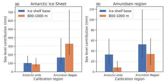
Figure 11. Projections of the sea level contribution of the AIS (a) and Amundsen Region (b) for SSP5-8.5 for all calibrated ESM-RF combinations using the quadratic parameterisation. The bars indicate the median sea level contribution in 2100 relative to 1995–2014. The thermal forcing and basal melt sensitivity are based on ocean temperature at two different depths: 100 m centred around the mean depth of the ice shelf base (blue) and 800–1000 m depth (orange). The black lines indicate the 17th–83rd percentiles.
