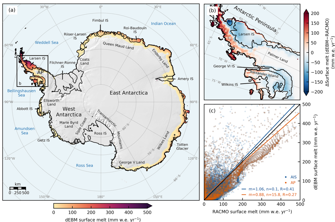
Figure 2. Present-day Antarctic surface melt rates computed by dEBM-simple and comparison to RACMO. (a) Map of mean 2005–2015 Antarctic surface melt rates (in millimeters water equivalent per year, mm w.e. yr -1 , as calculated with PISM-dEBM-simple in the calibrated historical run. Areas with melt rates below numerical significance (< 0.001 mm w.e. yr -1 ) are masked. AP, Antarctic Peninsula; IS, ice shelf. (b) Absolute difference of dEBM-simple minus RACMO-computed surface melt rates (in mm w.e. yr -1 ), averaged over the same period, shown for a zoomed-in section of the Antarctic Peninsula, the region with the highest average melt rates, indicated by the black square in panel (a). (c) Scatterplot of dEBM-simple versus RACMO-computed surface melt rates (in mm w.e. yr -1 ) and linear regression fits of the data (colored solid lines). Blue data points correspond to the whole Antarctic Ice Sheet (AIS) and orange data points to the zoomed-in section of the Antarctic Peninsula (AP) shown in panel (b). m and n are the slope and intercept of the regression lines, respectively, and R is the Pearson correlation coefficient. The black line marks the identity line.
