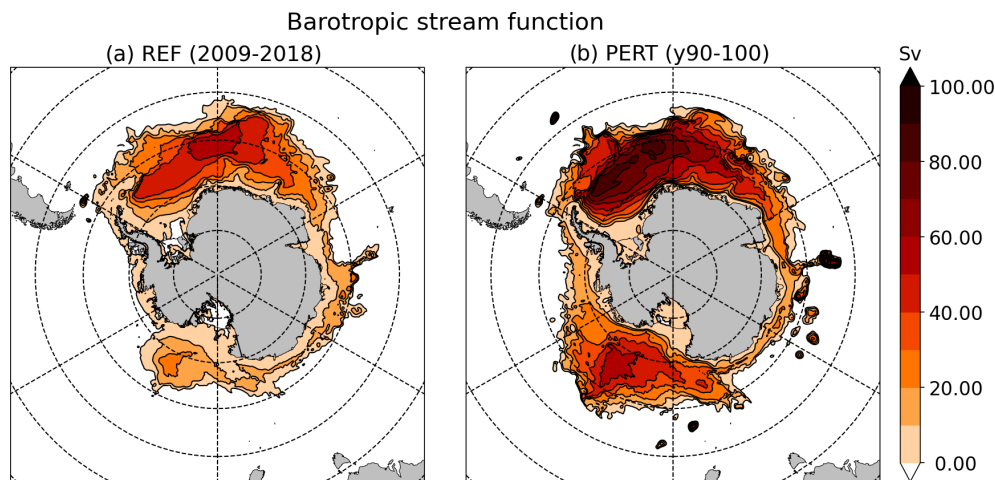
Figure 8. Climatological barotropic stream function in REF (a) and PERT (b). In white is the area beyond the polar gyres. Each contour is 10 Sv.
