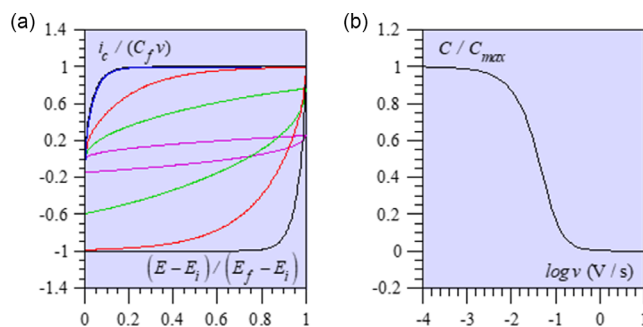
Figure 5. Charging characteristics of porous films. a) Dimensionless CV responses as a function of the adimensionalized scan rate, R_f C_f v / (E_f - E_i) = 0.1 (blue), 0.5 (red), 2 (green), 20 (magenta) ( v : scan rate, E_i , E_f : initial and inversion values of the cyclic potential scan). b) Charged capacitance versus the maximal capacitance as a function of the scan rate.
